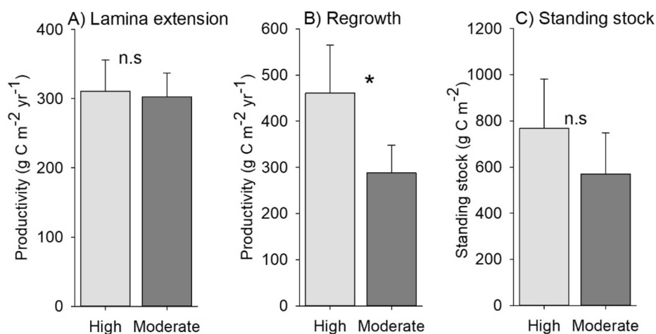
Figure 4. Mean ( \pm SE) values for NPP relating to (A) lamina extension and (B) regrowth into cleared areas and for (C) carbon standing stock for high wave exposure sites versus moderate wave exposure sites ('n.s.' indicates non-significant differences).
