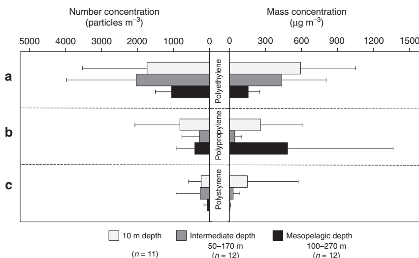
Fig. 4 Vertical distribution of microplastics in the study area. The bars show particle number ( \text{particles m}^{-3} ) and mass concentrations ( \mu\text{g m}^{-3} ) of a polyethylene, b polypropylene and c polystyrene averaged over all sampling stations at each depth horizon. Data presented as mean values with upper error bars (+1 s.d.) for clarity. In figure legend, letter n in parentheses indicates the number of stations sampled at the respective depth horizon (Supplementary Table 1 and Supplementary Data 1).
