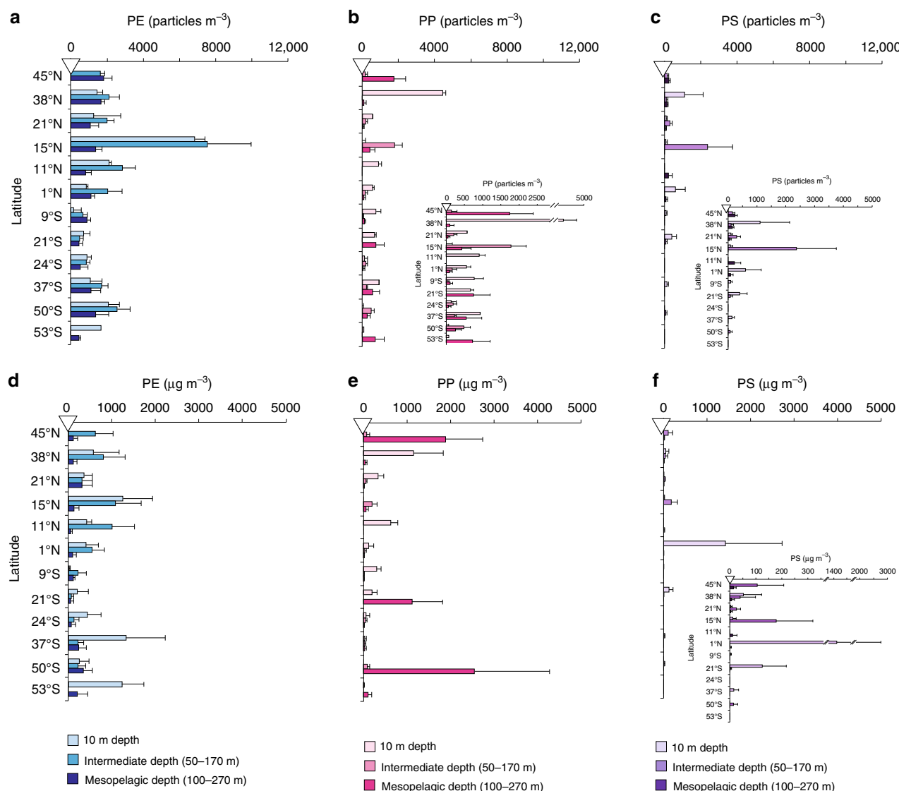
Fig. 2 Microplastics abundance in the study area. a–c particle number concentrations (particles m^{-3} ) and d, e mass concentrations ( \mu g m^{-3} ) of the polymer groups at each station and depth layer. No near surface (10 m) sample was taken at 45°N (marked with white triangle) due to pump failure. In a–c , the height of the bar shows the particle number concentration derived from the mean microplastic count in four imaged areas of a sample 24 and scaled to the known total area filtered and the known sample volume of the investigated sample fraction (see ‘Methods’ and Supplementary Data 1). In d–f , the height of the bar shows the mass concentration of microplastic derived from particle number concentration data and two-dimensional properties of detected individual particles using Method IV (ref. 10; see Supplementary Methods and Supplementary Data 1). All error bars are one standard deviation showing uncertainty propagated through the calculations. Only upper error bar (+1 s.d.) is shown for clarity. Note a magnified scale for concentrations of polypropylene ( b ) and polystyrene ( c, f ).
