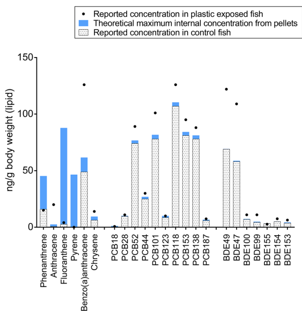
FIGURE 7: Calculated theoretical maximum lipid concentrations in marine plastic-exposed fish (blue bars) based on a mass balance analysis of reported initial marine pellet concentrations from Rochman et al. (2013b). Reported control fish (dotted bar) and marine plastic-exposed fish (black dots) lipid concentrations are also plotted. Fish were assumed to be 300 mg and the lipid content ranged from 2.1 to 6.2% (C. Rochman, University of Toronto, Toronto, Ontario, Canada personal communication).
