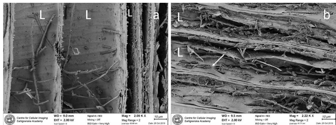
Figure 4. SEM micrograph shows growth and penetration of SR hyphae within and between the fibres. Hyphal growth takes place in the lumen (L). Here they divide and spread into the secondary cell wall and into adjacent fibres by penetration (a). Within the cell wall the hyphae orientates themselves along the direction of the microfibrils and starts to decompose the wood. Cavities with pointed ends are formed during decay (arrow) (b)—a decay feature more easily distinguished with LM-technique (Fig. 1a, b). Longitudinal section of sample BI1333 (a) and BI1332 (b).
