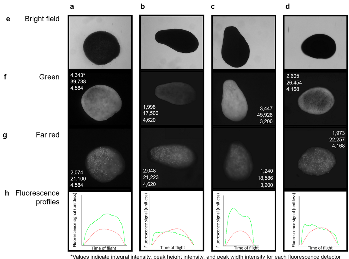
Figure 3. Brightfield (e), green (excitation 488 nm) (f) and far red (excitation 561 nm) (g) fluorescence micrographs, and corresponding fluorescence profiles (h) of four live Montipora capitata larvae (a–d) sorted with the COPAS VISION flow cytometer. Brightfield images (e) and fluorescence profiles (h) were obtained with the flow cytometer, and the fluorescence micrographs (f, g) were imaged using fluorescence microscopy. The three values on each fluorescence micrograph indicate the integral intensity, peak height intensity, and peak width intensity for each fluorescence detector. Time of flight in (h) has arbitrary units here, but can be used to calculate particle size due to the stable laminar flow and constant velocity of particle movement through the flow cell.
