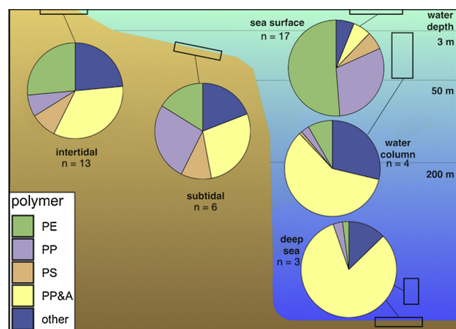
Fig. 5. Relative abundance of common polymer types in different sampling zone. Pie charts represent abundance data normalized to model predictions. For details see forest plots in supplementary information (Figs. S2–S5). PE: polyethylene; PP: polypropylene; PP&A: polyester, polyamide and acrylic; PS: polystyrene. Number of studies in each zone is indicated (n).
