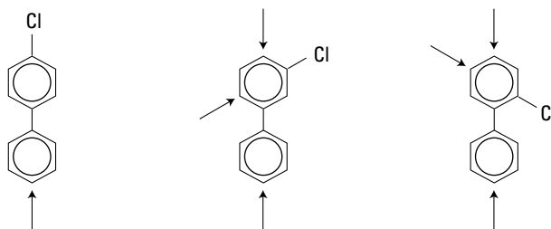
Figure 3.46. The preferred oxidation positions in a PCB molecule and the role of the chlorine position in the molecule in cytochrome P-450 catalyzed biotransformation reactions. From [147]. With permission.
