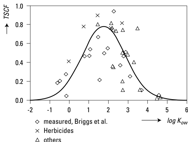
Figure 3.24. Transport of organic chemicals within plants as a function of K_{\text{ow}} ; adapted from Briggs et al. [81]. From: Trapp and Matthies [88]. With permission.
