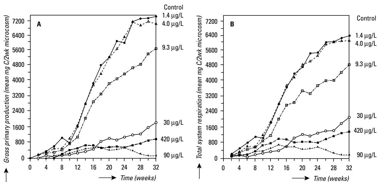
Figure 7.23. Bi-weekly gross primary production (A) and total system respiration (B) as measured in a microcosm test with copper. From Hedtkke [95]. With permission. Copyright Elsevier.
