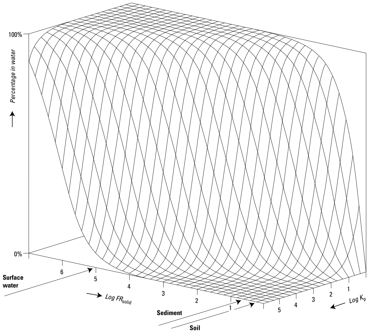
Figure 3.7. Fraction of a chemical in the water phase of a solid-water system as a function of the solid-water ratio ( FR_{solid} ) and the partition coefficient ( K_p ).
