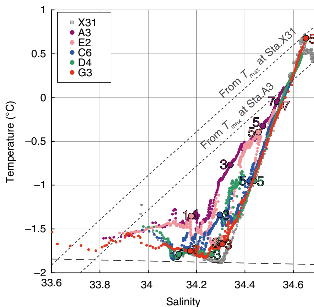
Fig. 3 Glacial meltwater signals on T-S space. Temperature-salinity relationships at five trough stations (Sta.A3, E2, C6, D4, and G3) with the northeast slope region (Sta.X31, shown by gray symbols). Two dashed diagonals denote theoretical mixing lines (“Gade line”) between glacier (ice) and observed mCDW temperature maxima (at Sta.A3 at the SGT ice front and Sta.X31 on the northeast slope region). Horizontal dashed line is the freezing point of seawater at atmospheric pressure. Numbers 1, 3, 5, 7 beside the large symbols indicate pressure levels at 100, 300, 500, and 700 dbar, respectively.
