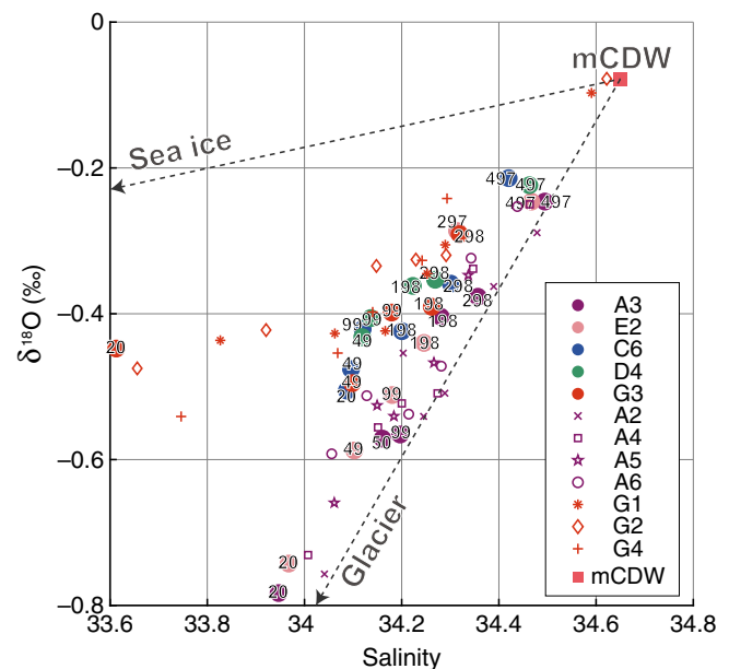
Fig. 4 Glacial meltwater signals on \delta^{18}\text{O} -S space. \delta^{18}\text{O} (the stable oxygen isotope ratio)-salinity relationships at five trough stations (colored circles with numbers showing the pressure where water samples were obtained), ice front stations (purple symbols), and mouth of LHB (red symbols). Two dashed lines extending from “mCDW” denote lines connecting two endmembers of “mCDW” with “glacier” and “sea ice”, respectively. Note that \delta^{18}\text{O} -salinity relationships for “glacier” and “sea ice” endmembers are beyond the range of plot.
