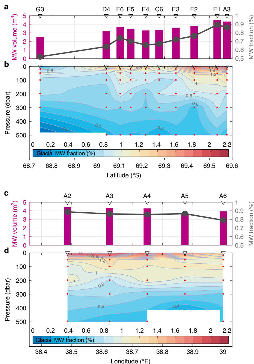
Fig. 5 Distribution of glacial meltwater. Column-integrated glacial meltwater volume per unit area (purple bar) and mean glacial meltwater fraction (%; line with dot) above 500 dbar ( a ) along- and ( c ) across-trough stations. Vertical sections of glacial meltwater fraction (%) ( b ) along- and ( d ) across-trough stations. Red dots indicate locations for water samples. The glacial meltwater fractions are linearly interpolated between water sample points and extrapolated from 20 dbar to sea surface. For Sta.G3, the extrapolation is conducted also from the deepest sampling layer to bottom.
