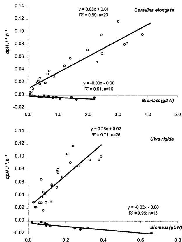
FIG. 2. – Hourly rate of pH variations per litre of seawater as a function of the biomass (in grams of dry weight, DW) of C. elongata and U. rigida (respectively) placed in experiment during light (open circle) and dark (dots).
