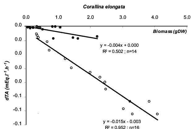
FIG. 4. – Hourly rate of total alkalinity (TA in mEq.l -1 ) per litre of seawater as a function of the biomass (in grams of dry weight, DW) of C. elongata placed in experiment during light (open circle) and dark (dots).
