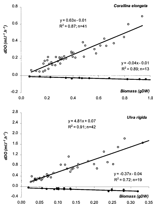
FIG. 1. – Hourly rate of dissolved oxygen variations in millilitres per litre of seawater (DO in \text{ml}\cdot\text{l}^{-1} ) as a function of the biomass (in grams of dry weight, DW) of C. elongata and U. rigida (respectively) placed in experiment during light (open circle) and dark (dots).
