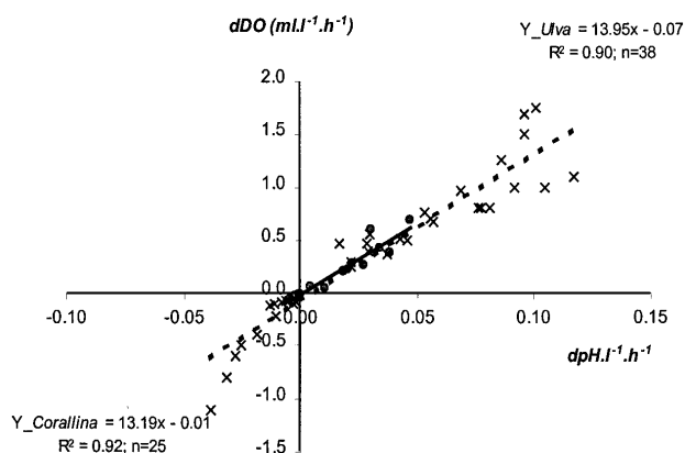
FIG. 3. – Regression plot between pH and DO variations of C. elongata (dots) and U. rigida (cross).
