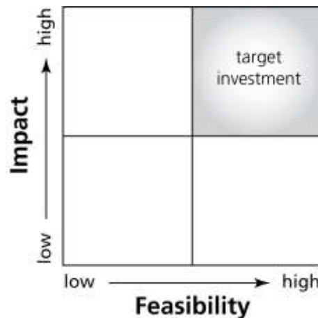
Figure 1. Essential Ocean Variables (EOVs) are those deemed 'essential' for understanding the ocean, having high impact in their contribution to understanding the ocean, and high feasibility to measure whilst addressing key scientific and societal issues [1]. This report focuses on the identification of ecosystem EOVS (eEOVs) that have high impact, although in most cases, further work is required to address the 'Readiness' of the monitoring system to ensure their sustained observation.
