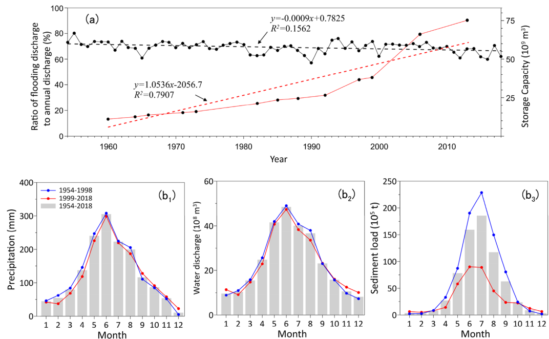
Figure 5. The ratios of flooding discharge to annual water discharge (black line) and total storage capacity (unit in \times 10^9 \text{ m}^3 ) for the reservoirs on the Pearl River (red line) (a). Monthly precipitation, water discharge, sediment load, and comparison between pre-abrupt and post-abrupt periods of sediment load in the Pearl River (b).
