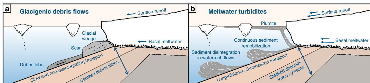
Fig. 1 Two types of sedimentary systems forming trough mouth fans. a Glacigenic debris flow dominated model implying temporarily stored sediment (glacial wedge) and non-disintegrating sediment transport. b Meltwater dominated model implying continuous channelized sediment transport in water-rich flows and surface plumites. Arrows indicating glacial meltwater are conceptual and not absolute values.
