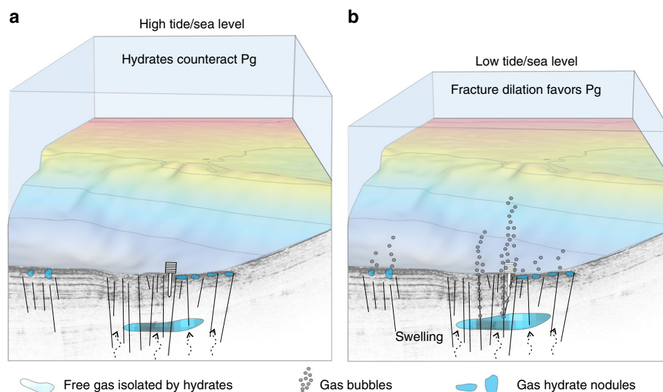
Fig. 7 Conceptual model of gas emissions. Schematic model showing how gas emissions may be affected by tides through fracture opening. a At high tides the system is under a balanced pressure field. b At low tides (<1 m water column height decrease) a subtle fracture dilation would shift the pressure field to favor gas advection and seepage. P_g stands for free gas pressure.
