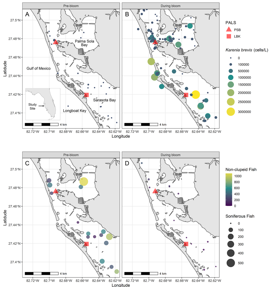
Figure 3. Locations of acoustic and red tide monitoring stations within the study site, along with the Karella brevis cell counts (A,B) and non-clupeid and soniferous fish catch per unit effort (C,D) pre- and during bloom. Maps were made in R v3.5.2 using the following packages: cowplot 55 , rnaturalearth 57 , sf 58 , tidyverse 59 , and viridis 60 and the Florida Shoreline (1 to 40,000 Scale) shapefile available from the Florida Fish and Wildlife Conservation Commission GIS & Mapping Data Downloads ( https://geodata.myfwc.com/ ) 61 . Note: one Karella brevis cell count (13,760,000 #/L recorded during the bloom at 27.42392 and -82.65965) was excluded from panel B as it was much larger than all other records and skewed the visualization of the data.
