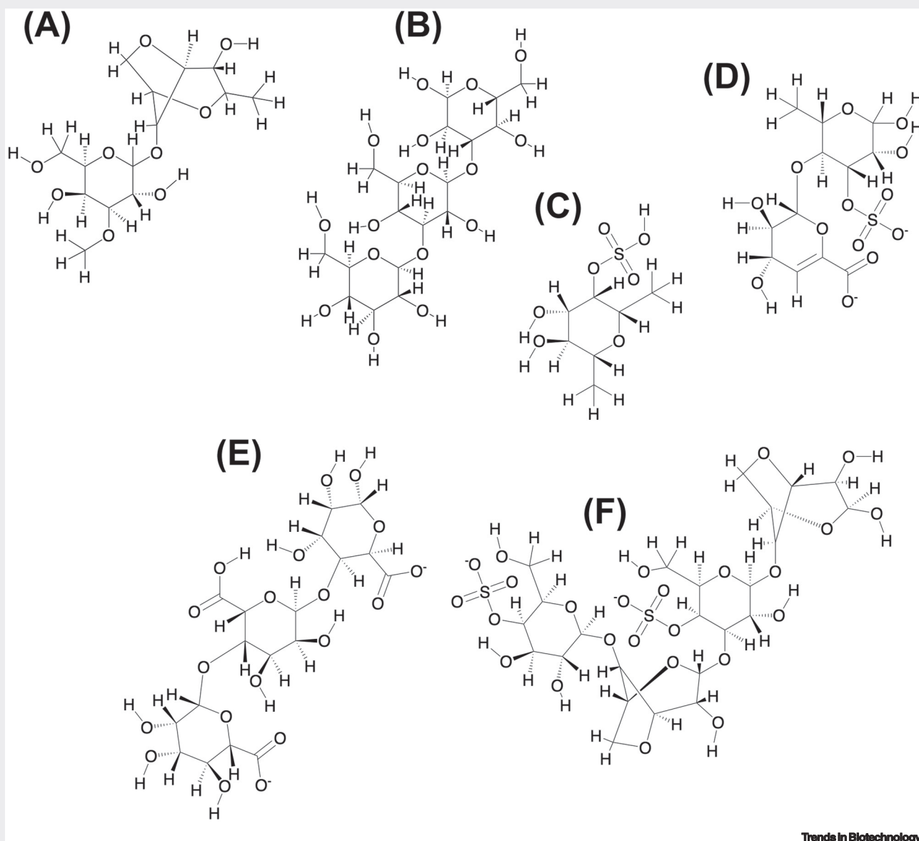
Figure II. Overview of Representative Chemical Structures of Major Representative Seaweed Polysaccharides. (A) Agar (shown as an arabinobiose dimer of galactose and 3,6-anhydro-L-galactopyranose); (B) laminarin (shown as a trimer of β-1,3 linked glucose); (C) fucoidan (shown as a sulfated fucan unit); (D) ulvan [shown as α-L-rhamnopyranose 3-sulfate (Rha3S), linked to β-D-glucuronate (GlcA)]; (E) alginate (shown as a trimer of mannuronic and guluronic acid, MGM); (F) carrageenan (shown as a tetramer of alternating 3-linked β-D-galactopyranose and 4-linked sulfated α-galactopyranose residues).
