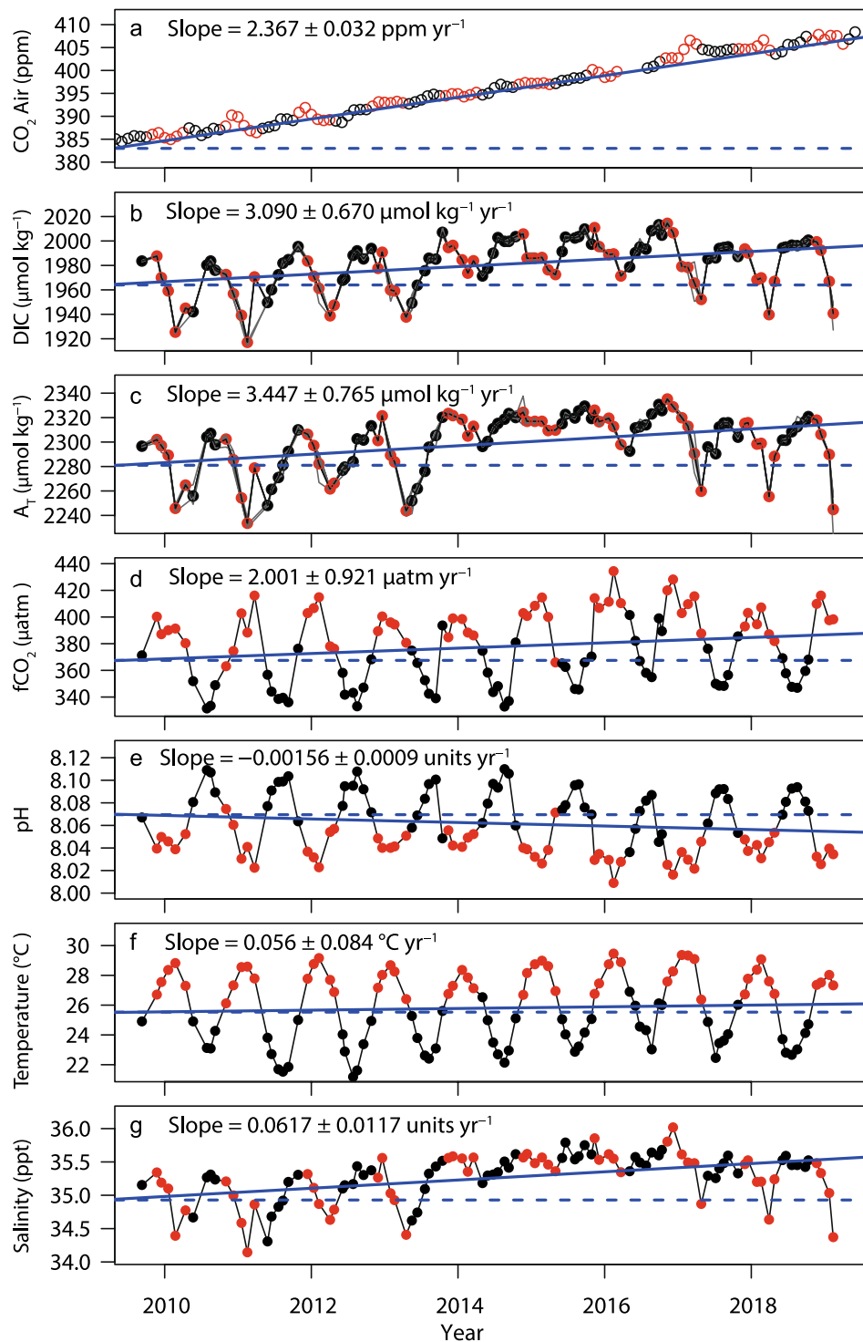
Figure 5. NRSYON: observed atmospheric CO 2 and seawater carbon chemistry values from 2009 to 2019. (a) Atmospheric CO 2 concentrations at the Cape Ferguson greenhouse gas monitoring station. (b) To (g): dissolved inorganic carbon (DIC), total alkalinity (A T ), temperature and salinity (all measured); fCO 2 and pH (calculated). Points are depth-averaged monthly seawater samples; red points indicate summer (November–April); black are winter (May–October). In (b,c) , the thin grey lines show the four sampling depths (0, 10, 20, 26 m). Straight solid blue lines are the linear trends, dashed blue lines are horizontal guides. Also shown are slopes of daily averaged data, unadjusted for changes in temperature and salinity.
