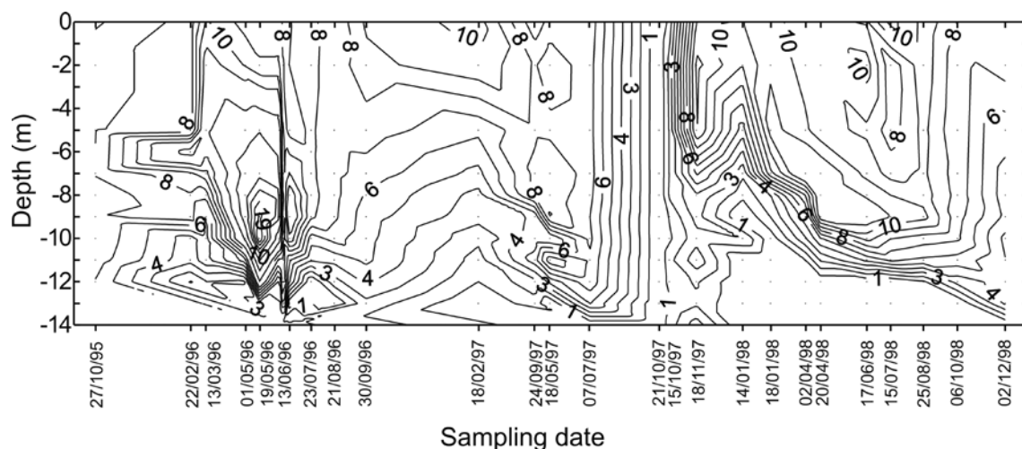
Fig. 4. Depth vs. time contour plots for oxygen concentrations (mg L -1 ) in the marine Lake Rogoznica
