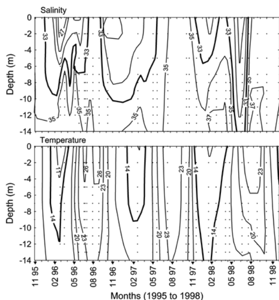
Fig. 2. Depth vs. time contour plots for salinity (PSU) and temperature (°C) in the marine Lake Rogoznica
