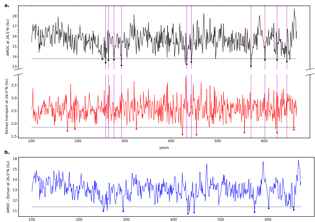
Figure 1. (a) Yearly-averaged time series of \Psi_M , i.e. the maximum value of the AMOC at 26.5°N (black) and of \Psi_E , i.e. the zonally integrated Ekman transport (red), respectively, in the pre-industrial control simulation of the model MIROC5. The dashed horizontal lines indicate, for each time series, the lower bound of the 2 \sigma confidence interval around the mean. The disks identify the time points at which extreme events occur, defined as the values extending below the threshold. Note that some of the values are not marked, because of the (10-year) clustering. The magenta vertical lines are drawn in correspondence with the extreme events of \Psi_M on top of both the time series. In this way, it is possible to qualitatively check whether a certain extreme event in the AMOC is related with anomalies in the wind-stress variations. (b) The difference time series \Psi_M^{cor} = \Psi_M - \Psi_E .
