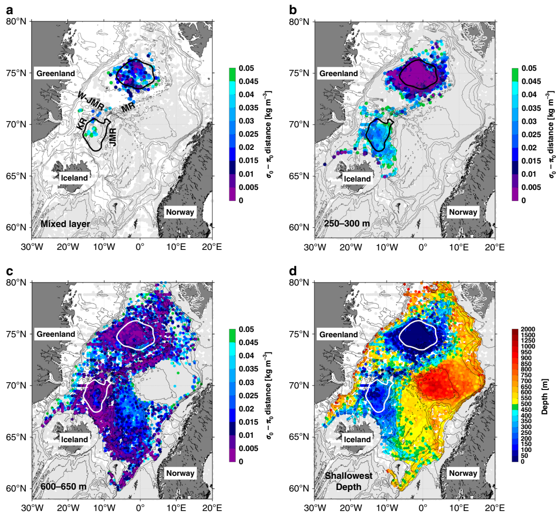
Fig. 2 Proximity in water mass space to the densest overflow water. a Distribution of the small potential density-potential spicity ( \sigma_0 - \pi_0 ) distances ( \leq 0.05 \text{ kg m}^{-3} ) for late-winter (February–April) mixed layers from 2005 to 2015. Distances > 0.05 \text{ kg m}^{-3} are shown by light-gray circles. The Greenland Sea and Iceland Sea gyres are delimited by the 4.5 and 7 dynamic cm contours, respectively, of sea surface dynamic height relative to 500 db (thick black and white contours). The thin gray contours show the bathymetry from ETOPO2, with four ridges labeled: MR, Mohn Ridge; W-JMR, West Jan Mayen Ridge; JMR, Jan Mayen Ridge; KR, Kolbeinsey Ridge. b, c The year-round distribution of small \sigma_0 - \pi_0 distances in the 250–300 m layer and 600–650 m layer, from 2005 to 2015. d The shallowest depth at which a small \sigma_0 - \pi_0 distance value ( 0.05 \text{ kg m}^{-3} ) is first found in the vertical. Stations where this value is not attained are shown by light-gray circles.
