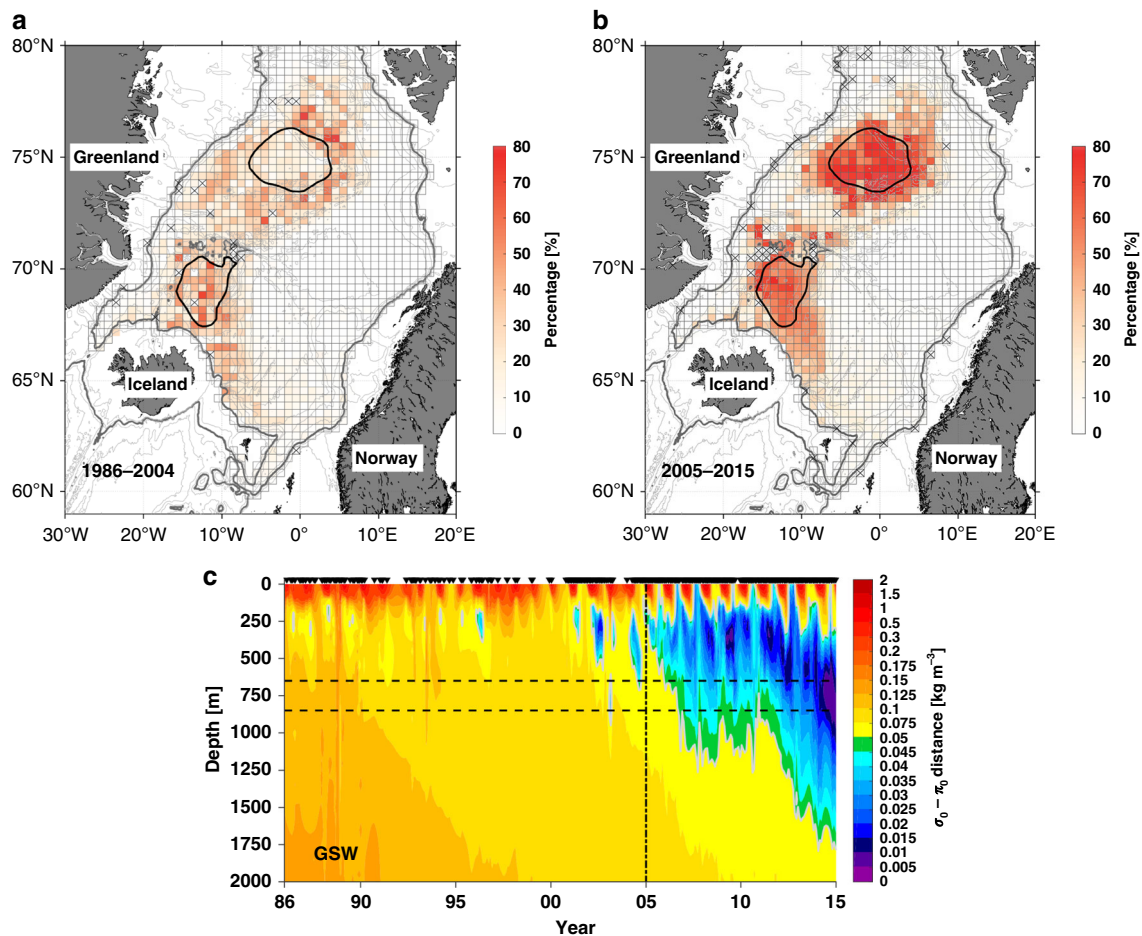
Fig. 5 Long-term variability of the densest overflow water. Relative layer thickness (in percentage, colors) of the small \sigma_0\text{--}\pi_0 distance water ( \leq 0.05 \text{ kg m}^{-3} ) in the upper 650 m of Nordic Seas for the time period (a) 1986–2004, and (b) 2005–2015. The thick gray contours show the 650 m isobath. The bins marked with an X denote the regions with no data coverage. c Evolution of \sigma_0\text{--}\pi_0 distances between the NIJ transport mode and the water within upper 2000 m of the Greenland Sea gyre (the black contour in a and b). The two horizontal dashed lines indicate the sill depths of Denmark Strait (650 m) and the Faroe Bank Channel (850 m). The vertical dashed line denotes year 2005. The gray contours denote \sigma_0\text{--}\pi_0 distances = 0.05 \text{ kg m}^{-3} .
