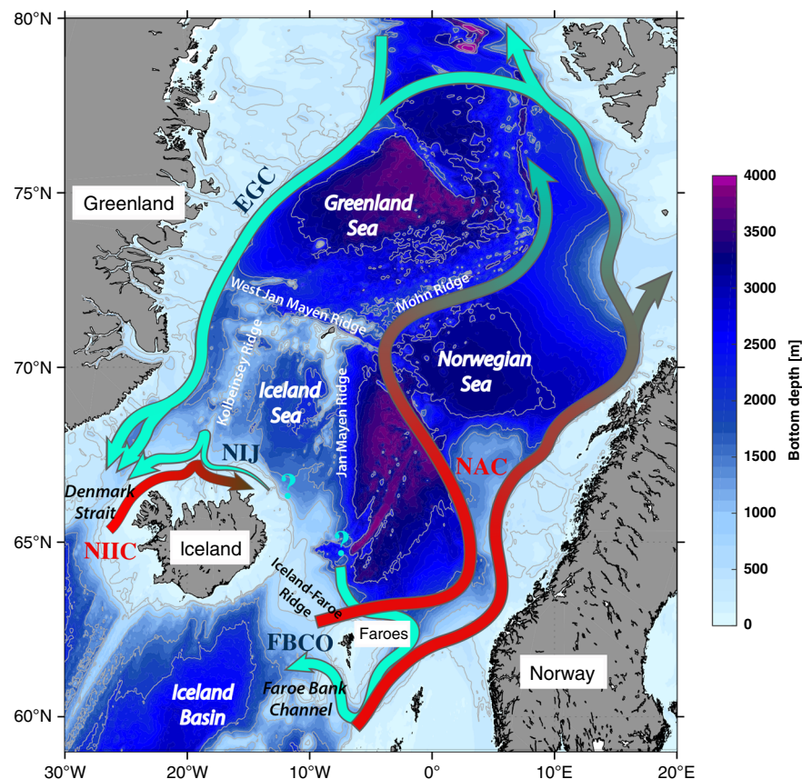
Fig. 1 Schematic circulation of the Nordic Seas. The pathways of warm Atlantic inflow and dense outflow are shown in red and green arrows, respectively. Colors and gray contours represent the bathymetry from ETOPO2, and the relevant ridges are named. NAC Norwegian Atlantic Current, NIIC North Icelandic Irminger Current, EGC East Greenland Current, NIJ North Icelandic Jet, FBCO Faroe Bank Channel overflow. Question marks denote uncertainty in the upstream source/pathways of the dense overflows.
