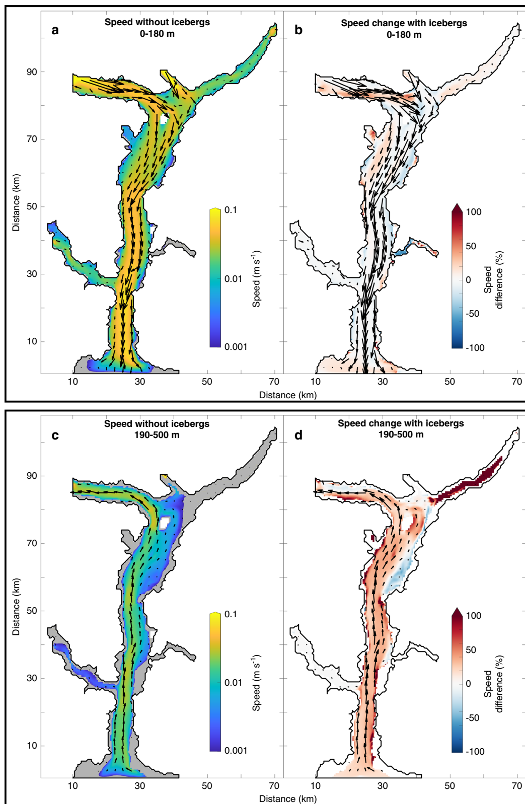
Fig. 5 The effect of icebergs on fjord circulation in our summer runoff forcing scenario. a Average current speed between 0 and 180 m depth in the no-iceberg simulation. b Relative speed change in the summer runoff forcing scenario compared to the equivalent no-iceberg simulation between 0 and 180 m depth, with positive values indicating an increase in speed. c, d As for a and b , but for the 190–500 m depth band. The arrows indicate the current velocity in the respective simulations averaged over the indicated depths. In all plots, the ocean boundary is at the bottom. Axis distances correspond to those in Fig. 1a.
