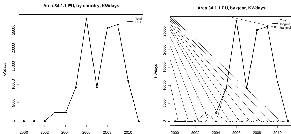
Figure 5.9.1.15.1. Deep Sea fishing effort (kW*days), 2000 – 2011, by country and by gear, in CECAF area 34.1.1 EU.
