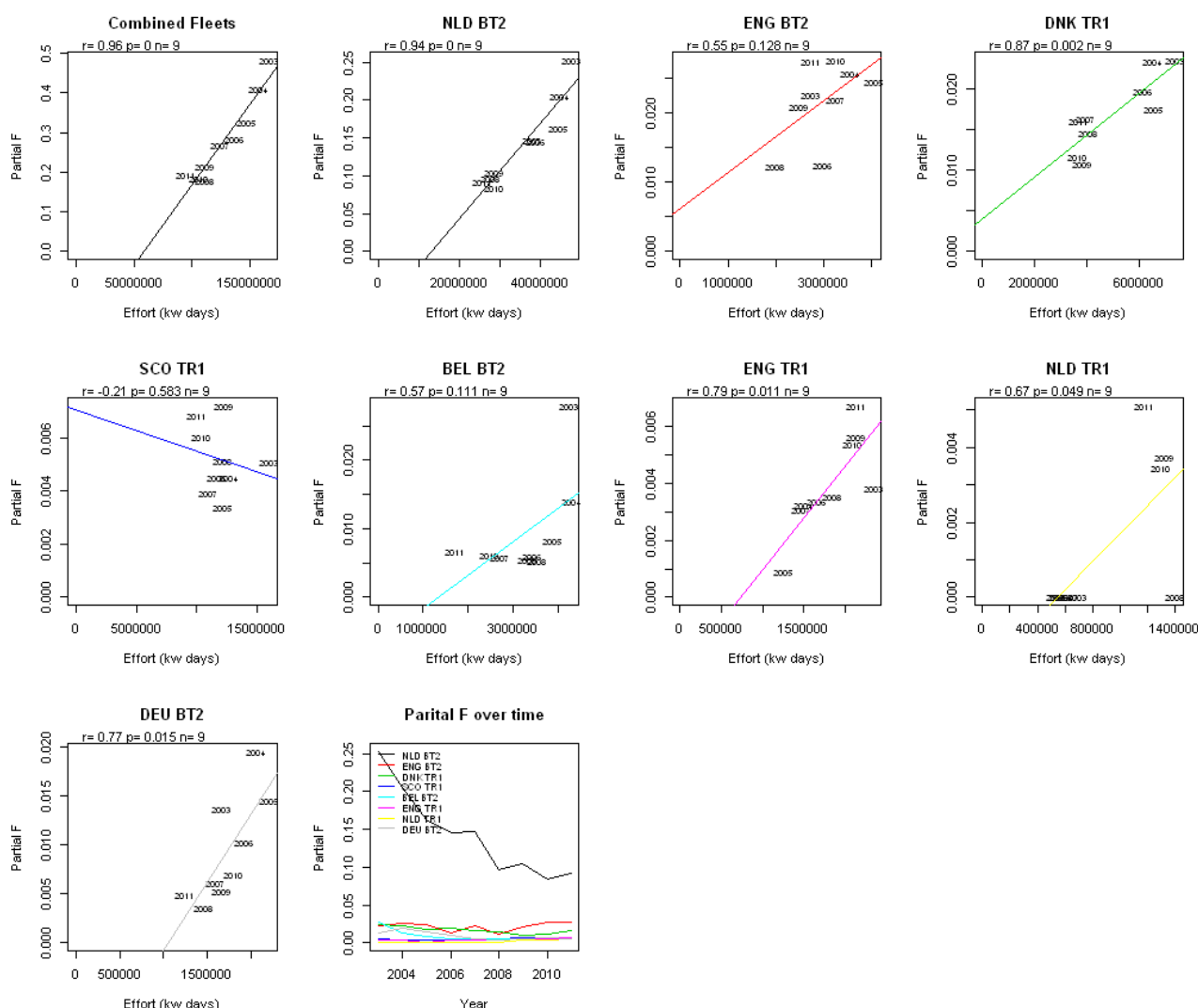
Fig. 5.3.14.4 Plaice. Partial fishing mortality (based on harvest rate estimates) over effort (kWd) in area 3b (North Sea) of major fisheries, 2003-2011. R = Pearson's coefficient of correlation, p value to quantify the statistical significance ( \leq 0.05 ). Note that the panel called combined fleets includes all regulated and unregulated fisheries and that the trends of the fisheries are not separated by special conditions.
