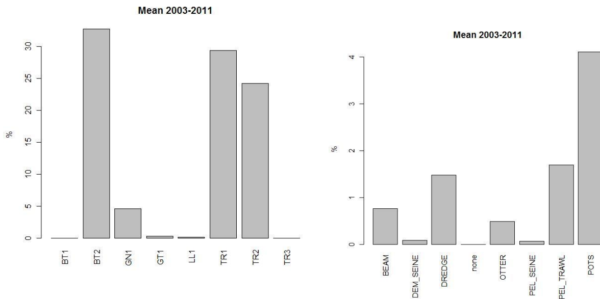
Figure 5.6.1.2.2. Contribution of each gear category to the total effort (kW*days) in the ICES Divisions VIIfg. Mean over 2003-2011.
