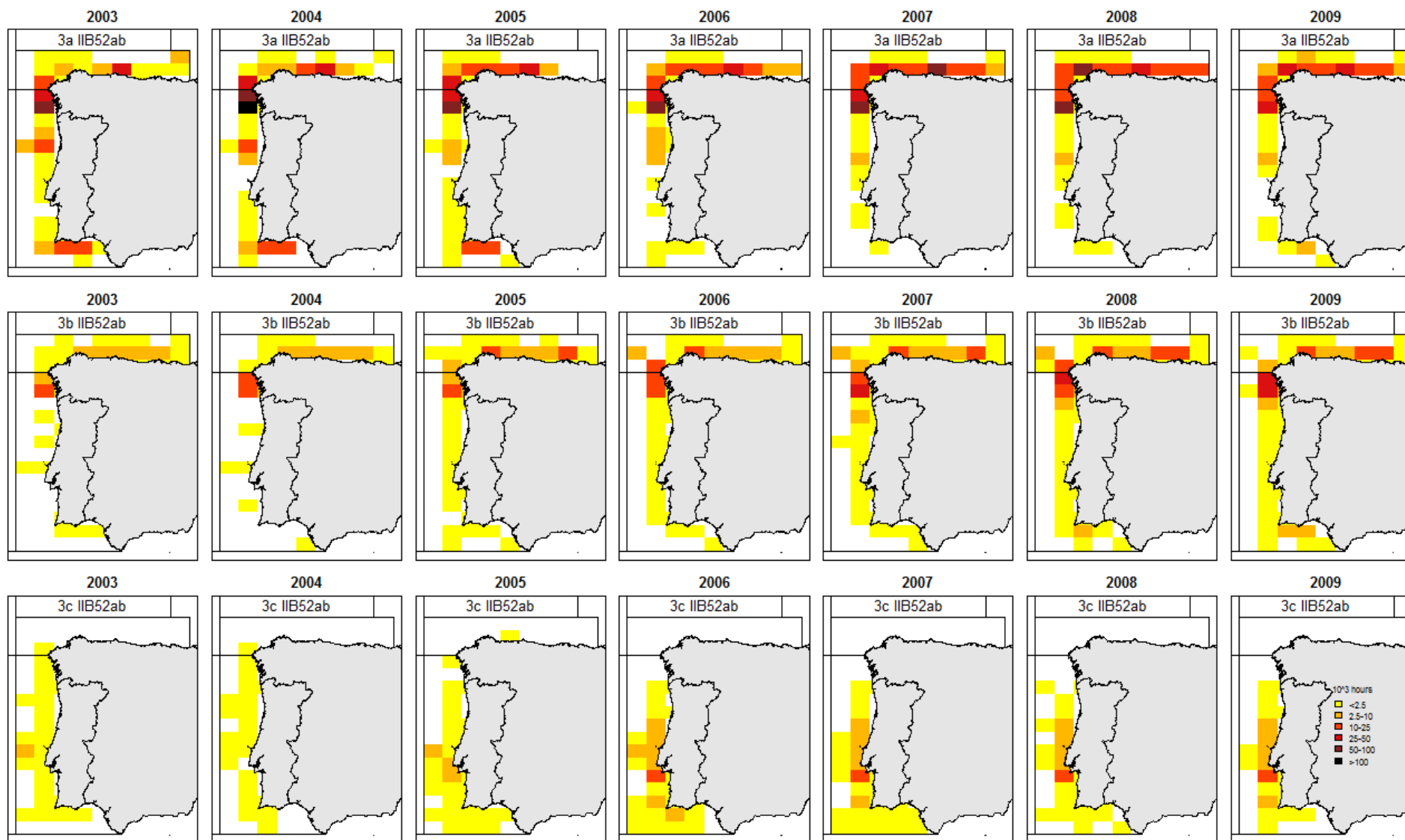
Figure 5.7.1.1.1 (II) Spatial distribution of effort by gear type with special conditions for the period 2003-2009. By mistake all Spanish effort under category “3c IIB52ab” was included in “3c none” in Figure 5.7.1.1.1(II), due to misallocation.
