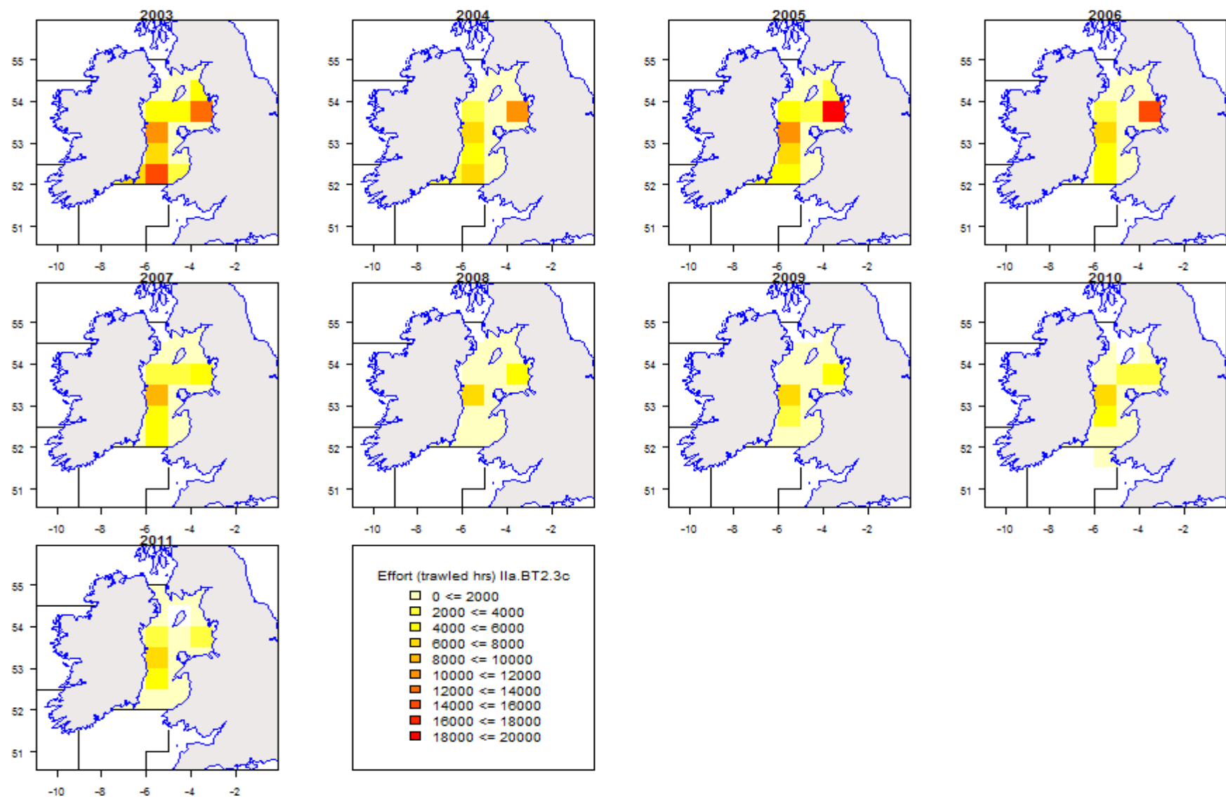
Figure 5.5.8.3. Irish Sea. Spatial distribution of effort (trawled hours) by ICES statistical rectangle for BT2, 2003-2011.
