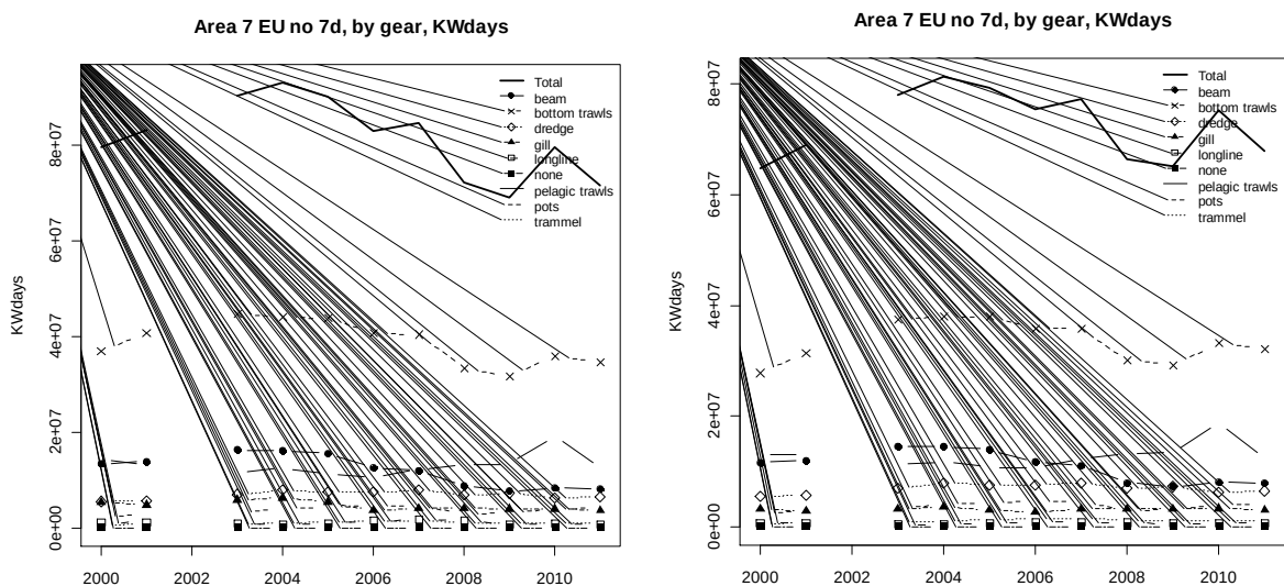
Figure 5.9.1.7.2.- Effort (kW*days) reported within ICES Sub-area VII EU no VIId by gear type, 2000-2011, with (left) and without (right) reported deepwater effort. Due to uncertainty in French 2002 data this year has been removed from the figures.
