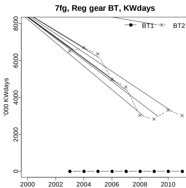
Fig. 5.6.1.2.5. Trend in nominal effort for beam trawl by mesh size range (Regulated Gear BT1, BT2) in the Celtic Sea (ICES Divisions VIIfg), 2003-2011.
