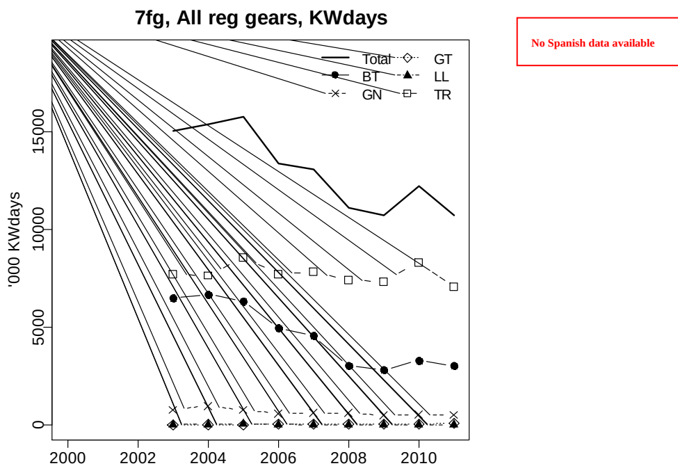
Fig. 5.6.1.2.3. Trend in nominal effort by gear types in the Celtic Sea (ICES Divisions VIIfg), 2003-2011.
