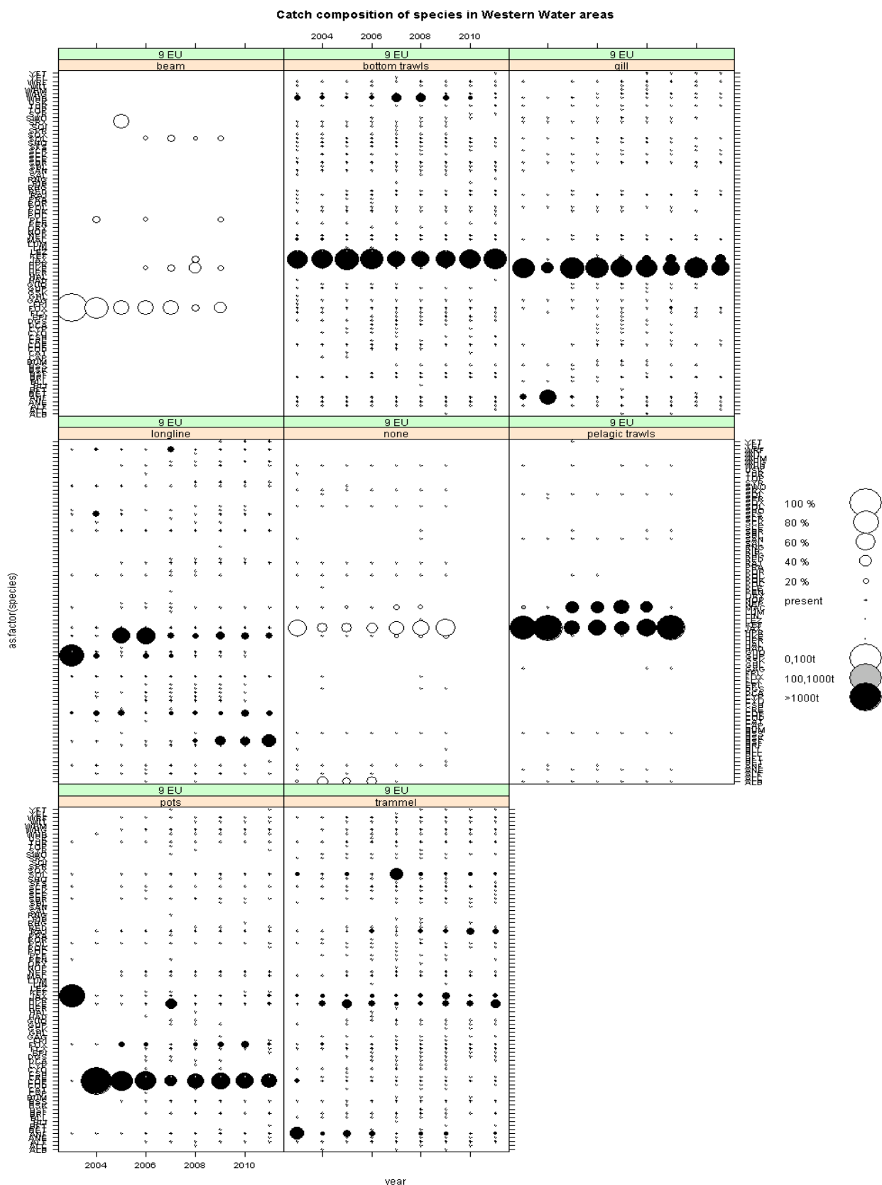
Figure 5.9.2.11.2. Landings composition by gear (countries combined) Western waters area IX EU. Size of circles represents relative contribution to landings, shading indicates quantity. Spanish 2010 landings not included. Note: Conclusions cannot be drawn from this graph due to major scaling errors within the Portuguese base data
