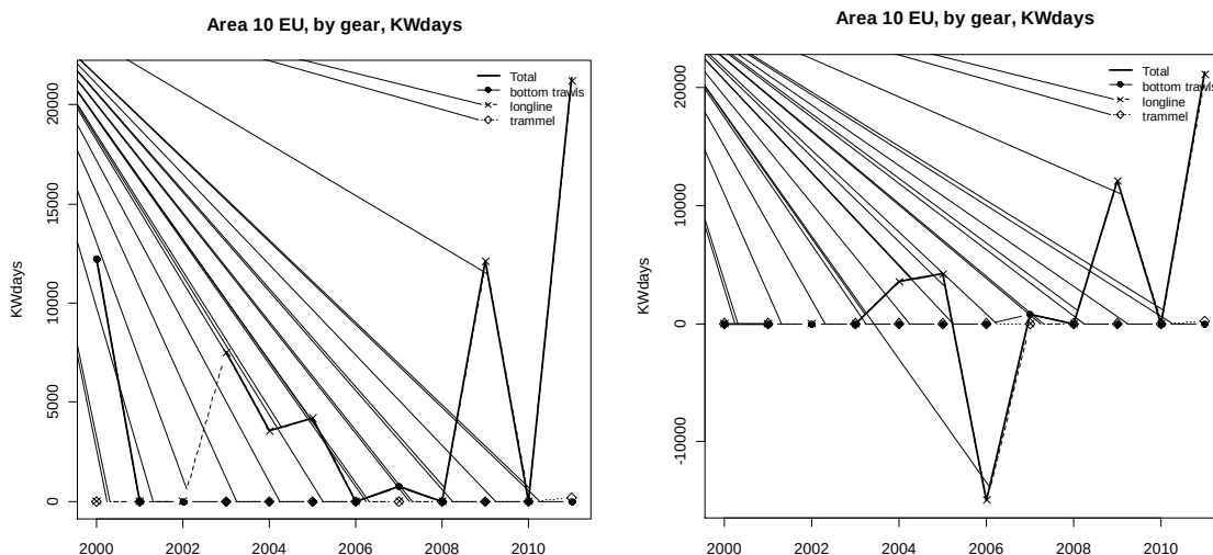
Figure 5.9.12.2.- Effort (kW*days) reported within ICES Sub-area X EU by gear type, 2000-2011, with (left) and without (right) reported deepwater effort.
