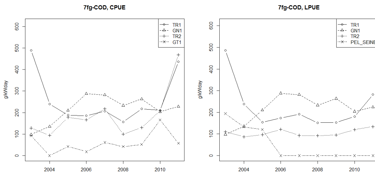
Figure 5.6.4.2.1 CPUE and LPUE for cod and for Divisions VIIIfg and for gear category and years 2003-2011.
