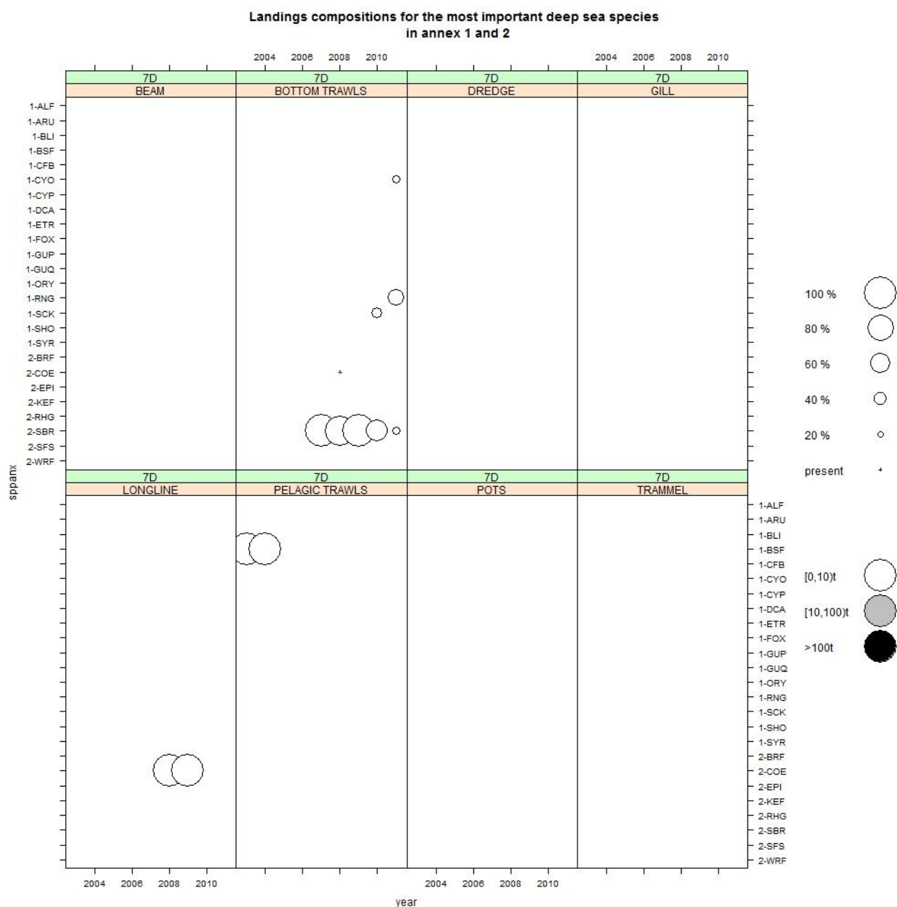
Figure 5.9.2.8.1. Landings of Annex 1&2 Deep Sea species (tonnes) 2003-2011 by gear ICES Area VII d
