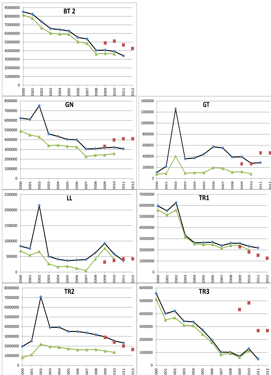
Figure 5.3.1.2.1 Management area 3b. Uptake of effort ceilings. Red squares: effort ceiling. Blue diamonds: regulated effort in whole area 3b (CPart 11 excluded). Green triangles : regulated effort in North Sea (ICES division IV) alone.
