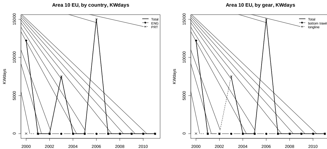
Figure 5.9.12.1. Deep Sea fishing effort (kW*days), 2000 – 2011, by country and by gear, in ICES Sub-area X EU.
