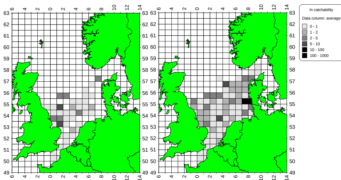
Fig. 5.3.15.5 Average cod catchability ( \ln(\text{CPUE})/(\ln(\text{NS IBTS Q1 index})) ) for the regulated gear BT2 (beam trawl 80-119mm) per rectangle in 2011 (left panel) and averaged for the period 2006-2011 (right panel). STECF EWG 12-12 notes that the resulting patterns of catchability in these specific management areas represent case studies and do not form the basis for any management advice.
