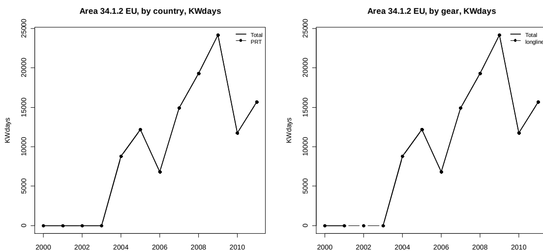
Figure 5.9.1.16.1. Deep Sea fishing effort (kW*days), 2000 – 2011, by country and by gear, in CECAF area 34.1.2 EU.
