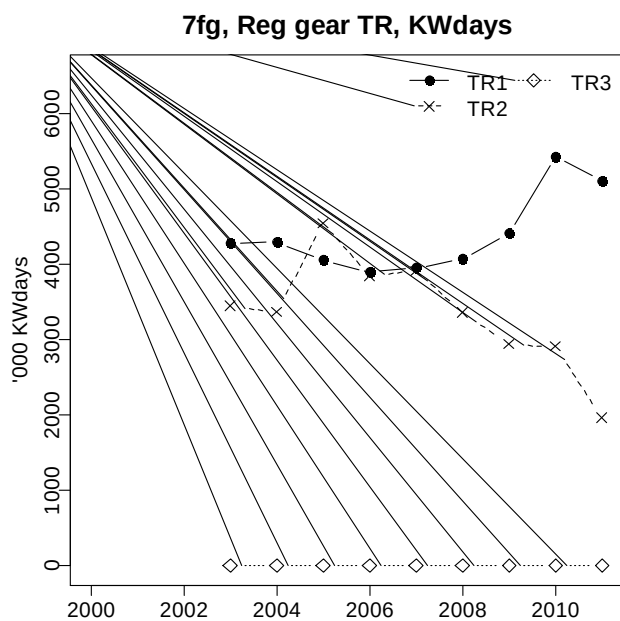
Fig. 5.6.1.2.4. Trend in nominal effort for demersal trawl (Regulated Gear TR1, TR2 and TR3) in the Celtic Sea (ICES Divisions VIIfg), 2003-2011.
