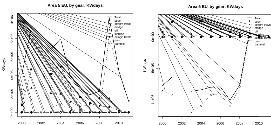
Figure 5.9.1.5.2.- Effort (kW*days) reported within ICES Sub-area V EU by gear type, 2000-2011, with (left) and without (right) reported deepwater effort.
