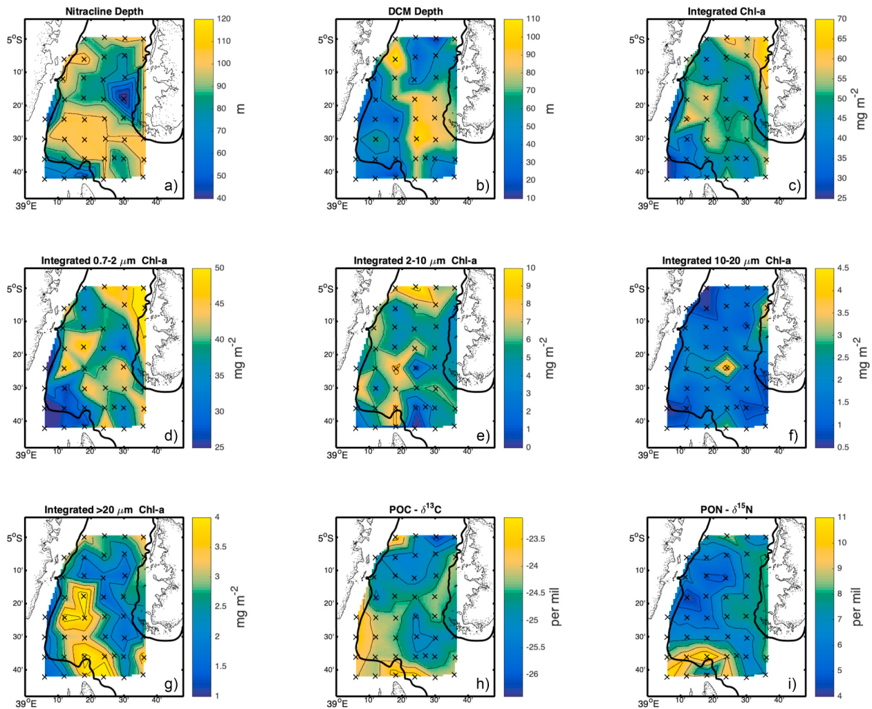
Fig. 7. Maps of a) nitracline depth ( 1 \mu\text{mol NO}_3^- \text{L}^{-1} contour), b) depth of deep chlorophyll maximum (DCM), c) integrated total chlorophyll-a, d) integrated picoplankton chlorophyll-a ( 0.7\text{--}2 \mu\text{m} ), e) integrated small nanoplankton chlorophyll-a ( 2\text{--}10 \mu\text{m} ), f) integrated large nanoplankton chlorophyll-a ( 10\text{--}20 \mu\text{m} ), g) integrated microplankton chlorophyll-a ( >20 \mu\text{m} ), h) particulate \delta^{13}\text{C} distribution, and i) particulate \delta^{15}\text{N} distribution.
