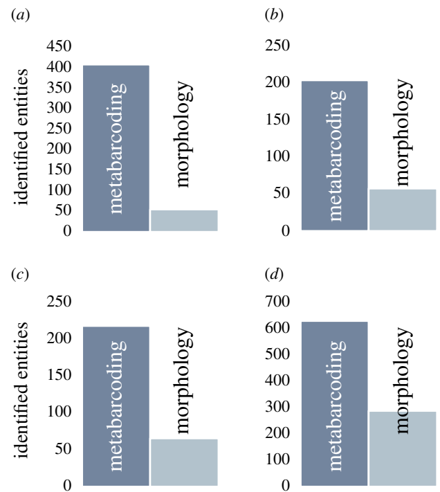
Figure 1. Higher diversities from bulk zooplankton samples using the metabarcoding approach (number of operative taxonomic units, OTUs) compared to morphological identification (identified to different taxonomic levels). (a) 18S V9 metabarcoding and morphological identification to family, order or phylum [109], (b) 18S V1–2 metabarcoding (97% similarity threshold) and morphological identification generally to species or genus level and in particular meroplanktonic larvae to major taxonomic groups [6], (c) 18S V7–V9 metabarcoding (97% similarity threshold) and morphological identification to species level or lowest-ranking taxon possible [115], (d) 18S V9 metabarcoding (97% similarity threshold) and morphological identification to genus level where possible [105].
