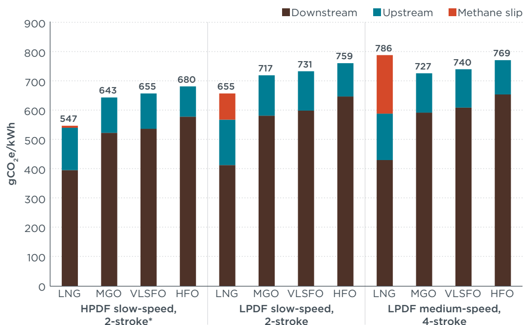
Figure 3: Life-cycle GHG emissions by engine and fuel type, 100-year GWP
