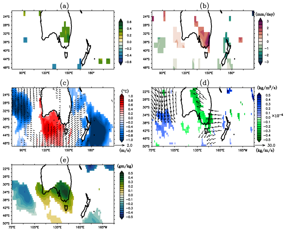
Figure 8. (a) Correlation field between IW4 and rainfall anomaly during austral summer. Composite of positive minus negative W4 extreme years in February (b) rainfall (in mm/day), (c) SST(shaded; in °C) and divergent wind at 850 hPa (vector; in m/s), (d) vertically integrated moisture divergence (shaded; in kg/m 2 /s) and moisture transport (vector; in kg/m/s) for whole atmosphere (i.e. surface to 1 Pa), and (e) vertically integrated specific humidity (in gm/kg) for whole atmosphere (i.e. surface to 1 Pa). Values less than 95% significance level are suppressed.
