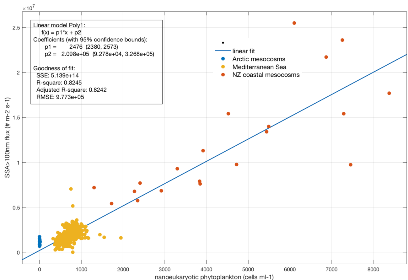
Figure 3. SSA larger than 100 nm flux number F_{\text{SSA100}} ( \# \text{ m}^{-2} \text{s}^{-1} ) calculated for a wind speed of 9 \text{ m s}^{-1} and 15^\circ \text{C} sea temperature as a function of the NanoPhyto (cells \text{ml}^{-1} ) from different regions. The solid line indicates the linear fit to the data set.
