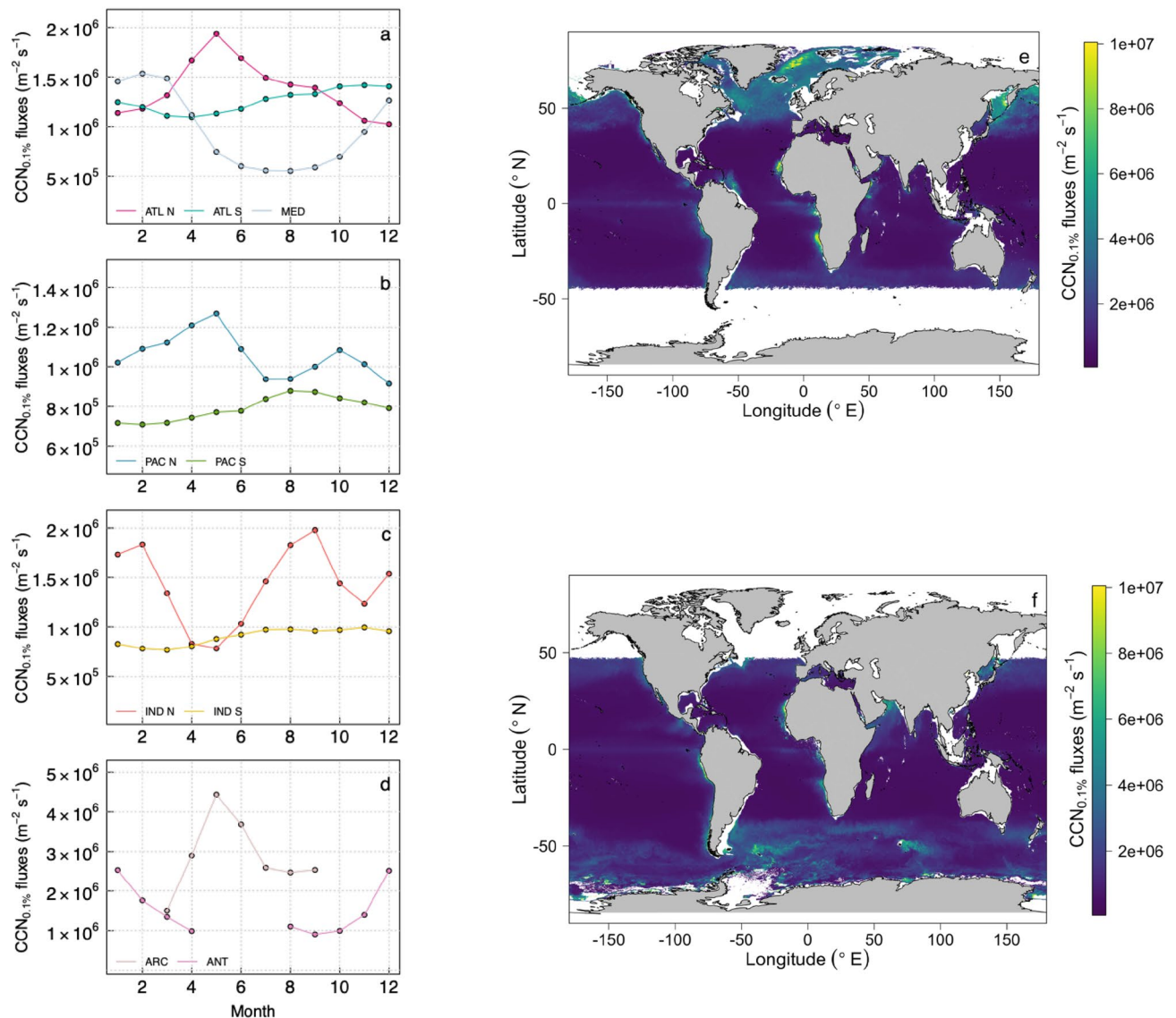
Figure 4. Global CCN 0.1% emission fluxes (m -2 s -1 ) computed for a 15 °C temperature from satellite-based nanoplankton cell abundance in June (e) and December (f). CCN fluxes were computed using Eq. (1), and assuming that CCN 0.1% is equal to SSA 100 . Median annual trends are represented for the different oceanic basins (a) ATL N: North Atlantic, ATL S: South Atlantic, MED: Mediterranean Sea; (b) PAC N: North Pacific, PAC S (South Pacific), (c) IND N (North Indian Ocean), IND S (South Indian Ocean), (d) ARC (Arctic Ocean), ANT (Southern Ocean). Maps provided (e,f) were created using R version 3.4.2. ( https://www.R-project.org/ ).
