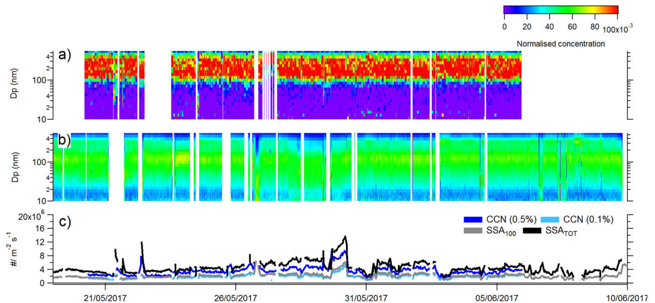
Figure 1. Time series along the PEACETIME (ProcEss studies at the Air-sEa Interface after dust deposition in The Mediterranean sea) ship track of (a) CCN 0.1% concentrations normalized to the sea spray concentration at given particle diameter (Dp). The activation diameter of SSA into cloud droplet at 0.1% supersaturation is visible at the change of colour from purple to red (b) sea spray concentration at given diameters (Dp) normalized with the total sea spray concentration, (c) flux of sea spray aerosol number (SSA TOT ), flux of sea spray larger than 100 nm number (SSA 100 ), and flux of CCN at 0.5% and 0.1% supersaturation, CCN 0.5% and CCN 0.1% , respectively.
