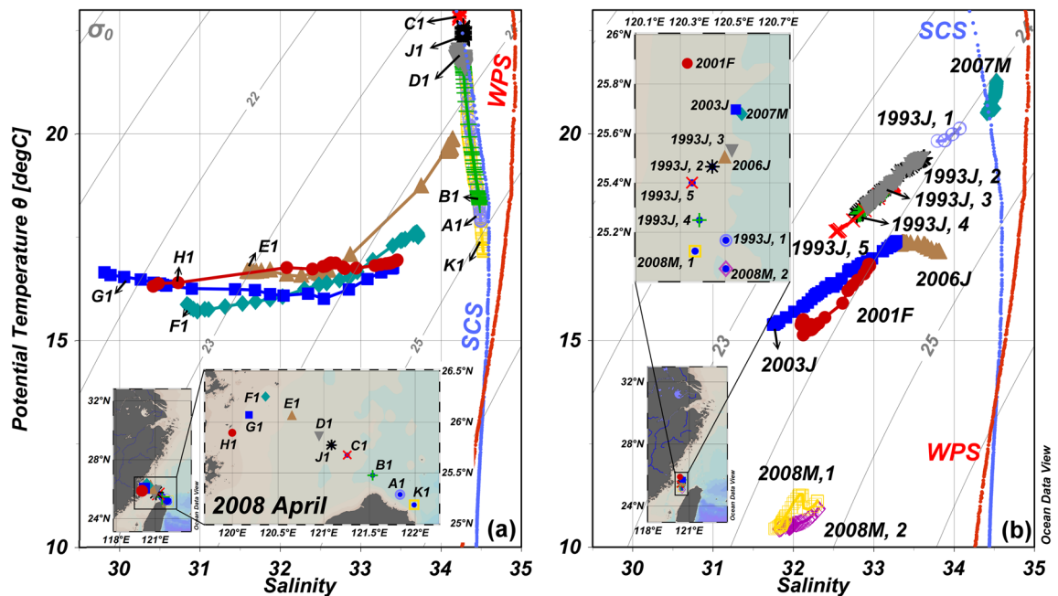
Figure 3. The \theta/S plots for the stations in the southwestern East China Sea: (a) ORI-861 data and (b) various other winter and spring data near Stn. E1 of the ORI-861 cruise (Station is identified by year and month: e.g., 2007 M denotes March, 2007; map generated by Ocean Data View version 5.2.1.; https://odv.awi.de ).
