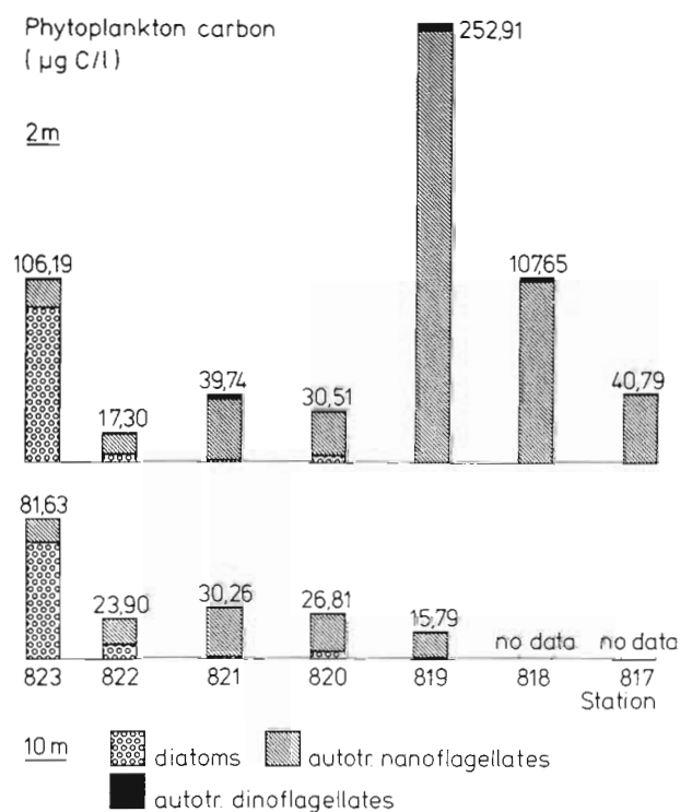
FIG. 5. — Phytoplankton biomass ( \mu\text{g C l}^{-1} ) and composition at two depths along the transect across the East Frisian tidal mixing front, showing frontal nanoflagellate peak at the surface of St. 819.
