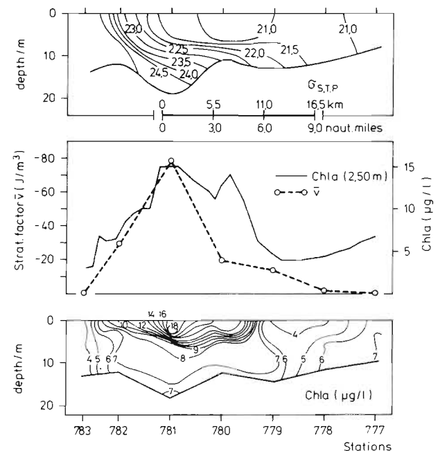
FIG. 2. — Elbe river plume front characteristics in May 1986. Top: Density section across the front. Middle: Variation of the stratification factor \bar{V} and of surface chlorophyll a . Bottom: Chlorophyll a isopleths.
