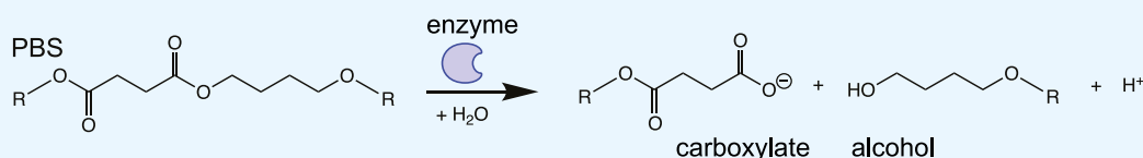
Figure 2.2b: Schematic of enzymatic hydrolysis of the aliphatic biodegradable polyester PBS under formation of the respective carboxylic acid and the alcohol. (Both figures adapted from Sander, 2019)
