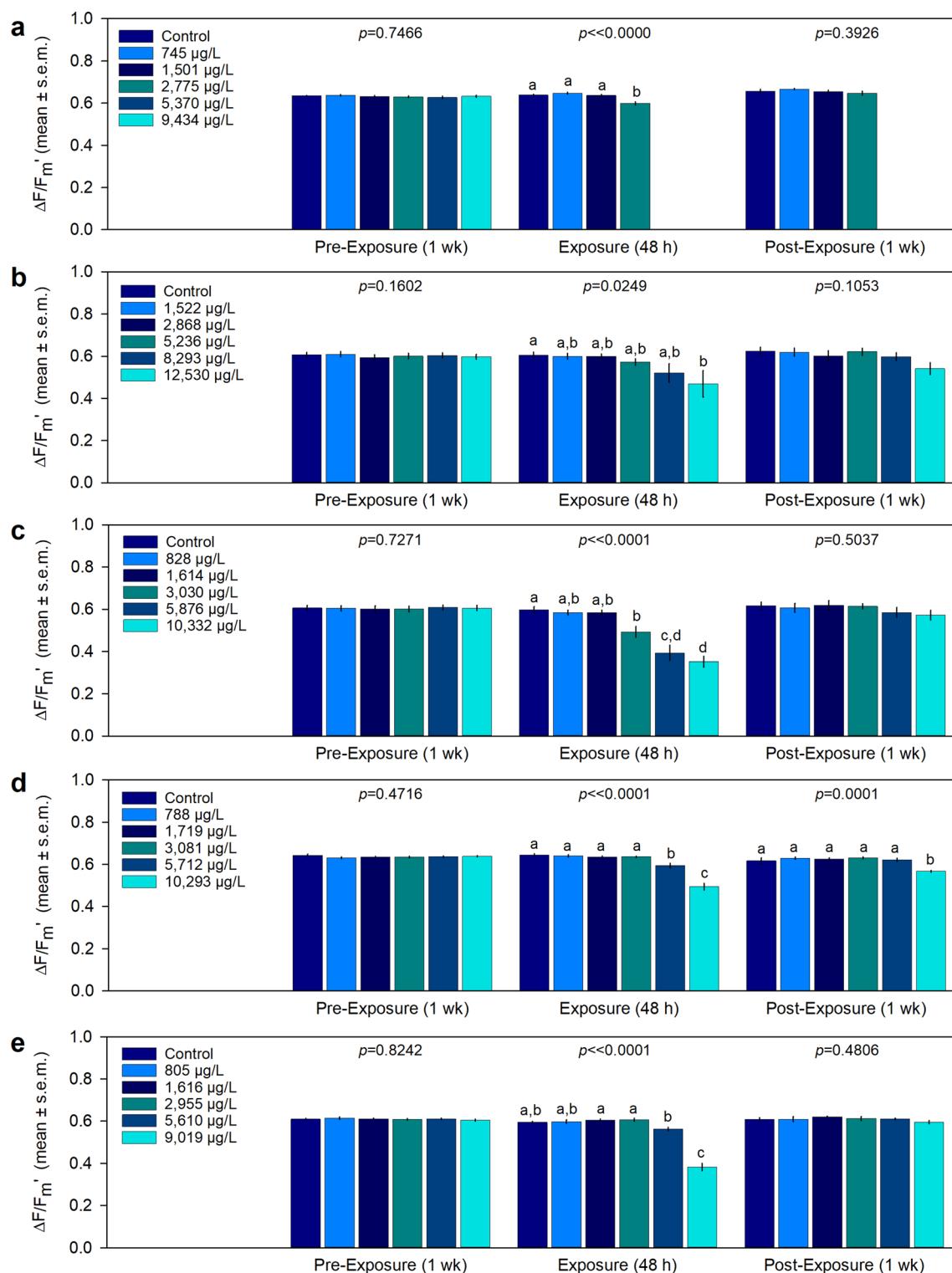
Figure 3. Light-adapted effective quantum yield (mean \pm s.e.m.) ( n=4 replicates) during the pre-exposure, exposure, and post exposure periods. (a) Acropora cervicornis , (b) Porites astreoides , (c) Siderastrea siderea , (d) Solenastrea bournoni , and (e) Stephanocoenia intersepta . Letters above each bar represent statistical differences between treatments at each time point (a–c; \alpha=0.05 ).
