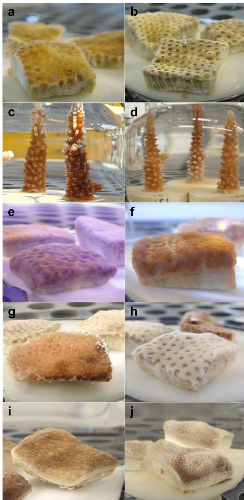
Figure 1. Typical physical changes at various time points in response to 1-methylnaphthalene (1-MN) exposure. (a) Solenastrea bournoni , control coral @ T1, and (b) polyp retraction in the 10,293 \mu\text{g L}^{-1} 1-MN treatment @ T1; (c) Acropora cervicornis , control coral @ T12, and (d) elevated mucus production in the 9434 \mu\text{g L}^{-1} 1-MN treatment @ T12; (e) Siderastrea siderea , control coral @ T8, and (f) tissue swelling in the 3030 \mu\text{g L}^{-1} 1-MN treatment @ T8; (g) Stephanocoenia intersepta , control coral @ T36, and (h) bleaching in the 1616 \mu\text{g L}^{-1} 1-MN treatment @ T36; and (i) Porites astreoides , control coral @ T36, and (j) tissue loss/mortality in the 12,530 \mu\text{g L}^{-1} 1-MN treatment @ T36.
