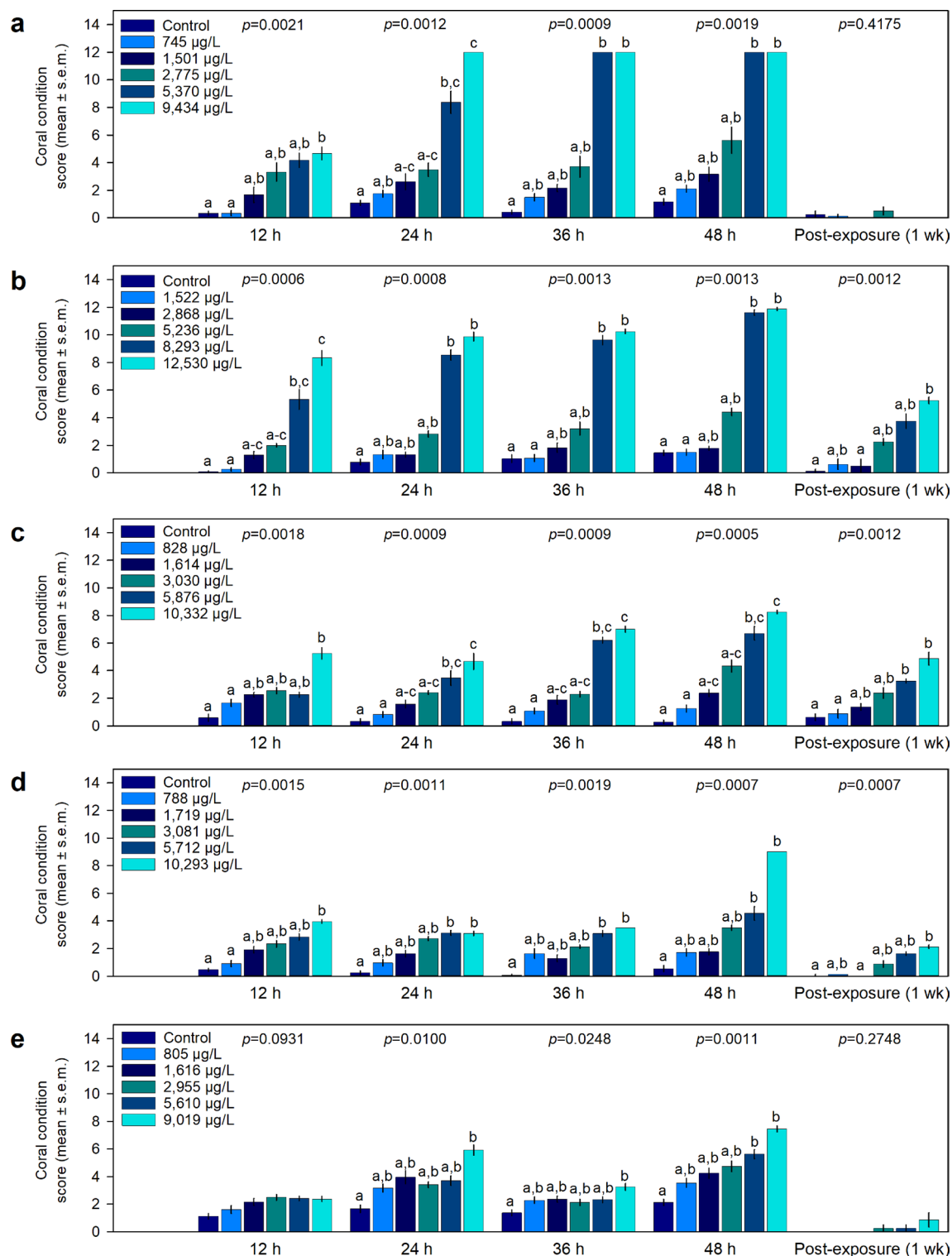
Figure 2. Coral condition scores (mean \pm s.e.m.) (n=4 replicates) during 1-methylnaphthalene exposures at 12 h, 24 h, 36 h, 48 h and 1 week post-exposure. (a) Acropora cervicornis , (b) Porites astreoides , (c) Siderastrea siderea , (d) Solenastrea bournoni , and (e) Stephanocoenia intersepta . Letters above each bar represent statistical differences between treatments at each time point (a–c; \alpha=0.05 ).
