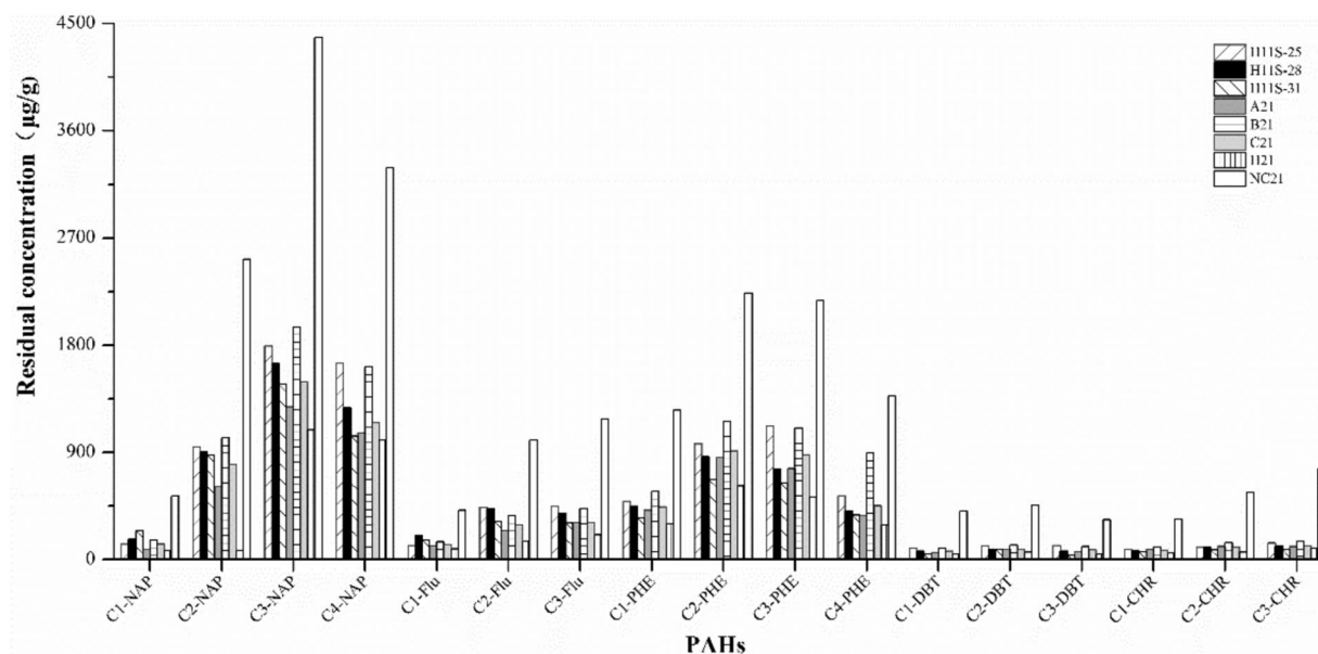
Figure 6. The n-alkanes and PAHs residual concentration in the crude oil after biodegrading 21 days by isolated strains and consortia ( a n-Cm: alkane with m carbon atom, for instance, n-C16 is alkane with 16 carbon atom; "PR" is pristane, "PH" is phytane. b NAP, FLU, DBT, PHE, and CHR represent for naphthalene, fluorine, dibenzothiophene, phenanthrene, chrysene, respectively. C1(C2, C3, C4)-NAP, alkylated naphthalene with straight-chain of 1 ~ 4 carbon atoms; C1(C2, C3)-FLU, alkylated fluorene with straight-chain of 1 ~ 3 carbon atoms; C1(C2, C3)-DBT, alkylated dibenzanthrene with straight-chain of 1 ~ 3 carbon atoms; C1(C2, C3, C4)-PHE, alkylated phenanthrene with straight-chain of 1 ~ 4 carbon atoms; C1(C2)-CHR, alkylated chrysene with straight-chain of 1 ~ 2 carbon atoms).
