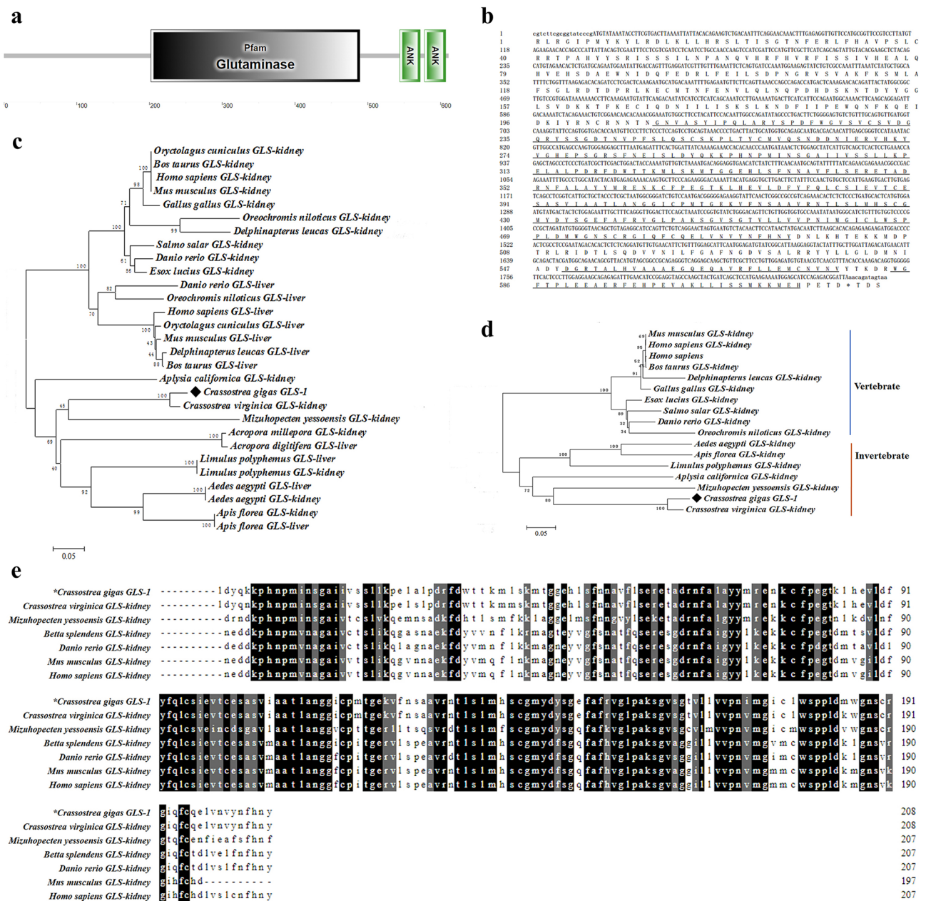
Figure 1. The sequence characteristics of CgGLS-1. (a) The structure of CgGLS-1 predicted by SMART. CgGLS-1 protein contains a Glutaminase domain (202–489 aa), and two ANK domains (544–607 aa). (b) The ORF of CgGLS-1. The GLS domain and ANK domains are underlined. (c,d) The Neighbor-joining (NJ) phylogeny tree of GLS-1 from various species including vertebrates and invertebrates. The information of sequences used for the CgGLS-1 phylogenetic analysis was shown in Table 2. The bootstrap value is displayed by the numbers at the forks. (e) Multiple sequences alignment of CgGLS-1 with other GLS from vertebrates and invertebrates. The black shadow region indicates positions where all sequences share the same amino acid residue. Similar amino acids are shaded in grey. The information of sequences used for the CgGLS-1 alignment is shown in Table 2.
