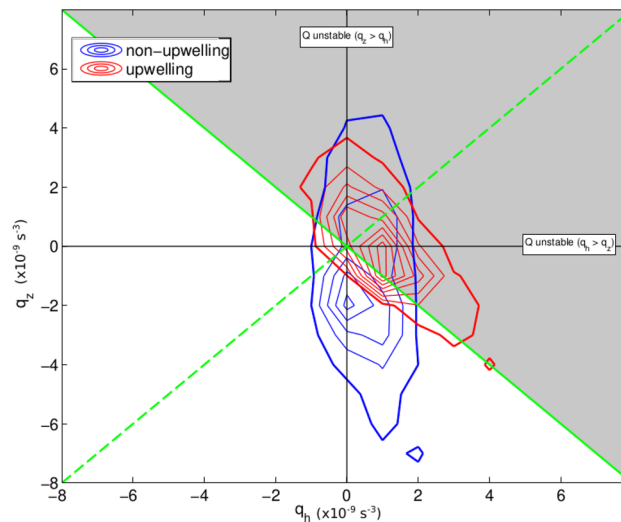
Figure 5. Comparison of horizontal and vertical potential vorticity during upwelling and non-upwelling periods. A 2d-histogram of q_h and q_z ( s^{-3} ) for upwelling (red) and non-upwelling (blue) periods for the area between 0-1^{\circ}\text{S} , 93-91^{\circ}\text{W} . 1% of values contour is indicated using a thicker line. Q=0 (i.e. q_h + q_z = 0 ) is marked as a thick green line, and q_h = q_z is indicated as a dashed green line. The area of parameter space favourable to the development of submesoscale instabilities is shaded grey.
