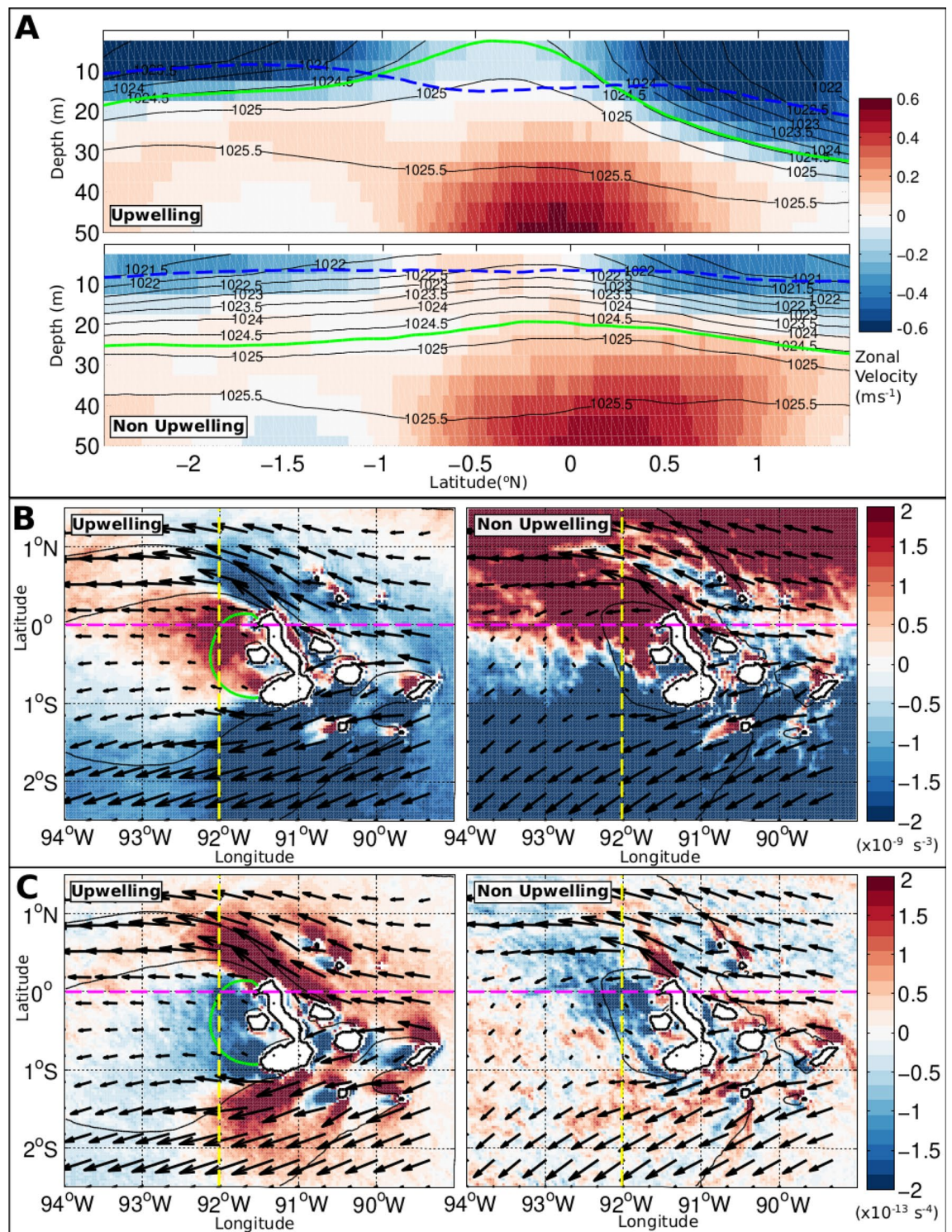
Figure 3. Model stratification and potential vorticity during upwelling and non-upwelling periods. (A) A section along 92^\circ\text{W} of mean zonal velocity, with density contours (black), mixed layer depth (blue), and 20^\circ\text{C} isotherm (green) means for periods of upwelling and non-upwelling conditions. (B) Full potential vorticity ( Q , \text{s}^{-3} ) averages for upwelling and non-upwelling periods, along with period-mean surface velocity vectors in black, where water speeds are in the range 0.01\text{--}0.83 \text{ m s}^{-1} for upwelling periods and 0.01\text{--}0.73 \text{ m s}^{-1} for non-upwelling periods. (C) Q flux vector ( J_z^F , \text{s}^{-4} ) and mean surface velocity vectors in black for upwelling and non-upwelling periods. The location of the density section shown in panel (A) is marked as a yellow dashed line, and the equator as a magenta dashed line.
