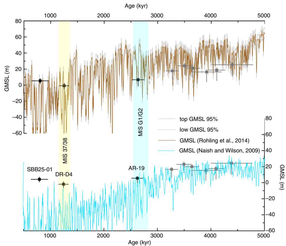
Figure 3. Pliocene and Pleistocene global mean sea level estimates. POS-derived Pliocen and Pleistocene GMSL are indicated by silver 34 and black (this study) markers, respectively (age uncertainties are 2\sigma ; the GMSL of the marker corresponds to the mode and the error bars to the 16th and 84th percentiles). Thermal expansion correction is not applied for any of these estimates. Brown and cyan curves show two oxygen isotope based sea level reconstructions (brown is the GMSL derived estimates from the planktonic foraminifera and the marginal basin residence time 24 and cyan is the GMSL curve derived from the conversion of LR04 benthic foraminiferal \delta^{18}\text{O} stack by scaling with a calibration of 0.011 \text{ ppt m}^{-1} as in 23 ).
