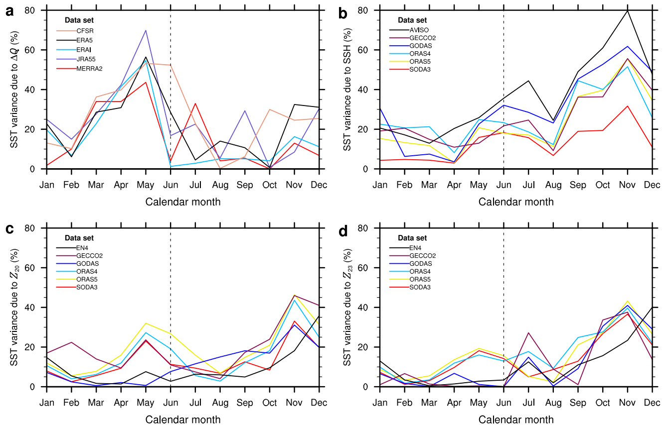
Fig. 2 Sea surface temperature explained variances. The explained variances were estimated from r^2 and expressed as percentages: where r is the correlation between the seasonally stratified Atl3 SST (that is, average in the region 3^{\circ}\text{N} – 3^{\circ}\text{S} , 0^{\circ} – 20^{\circ}\text{W} ) and a diabatic-heating gradient ( \Delta Q ), b sea surface height (SSH), c 20^{\circ}\text{C} isotherm depth ( Z_{20} ) and d 23^{\circ}\text{C} isotherm depth ( Z_{23} ) averaged over the equatorial Atlantic ( 3^{\circ}\text{N} – 3^{\circ}\text{S} , 5^{\circ}\text{E} – 40^{\circ}\text{W} ).
