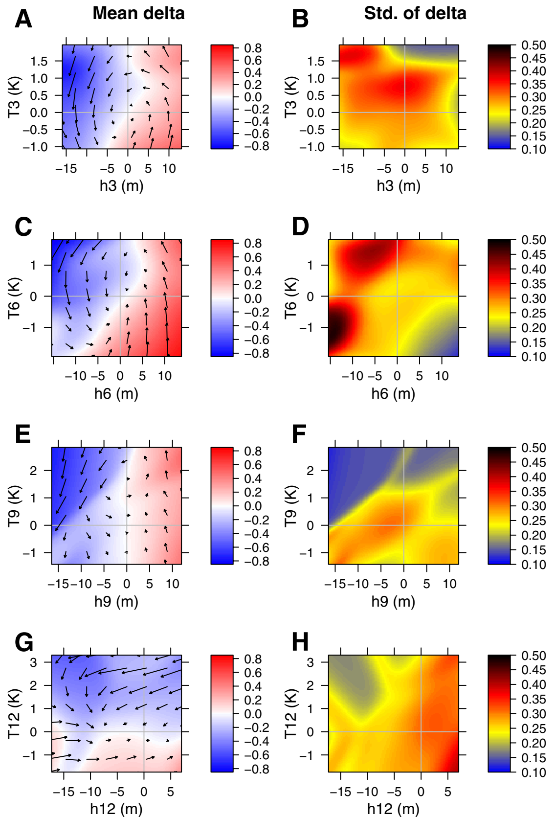
Figure 1. (Left) Mean tendency of SST anomalies in the Niño 3 region for different months (color) [K month -1 ], as a function of Niño 3 SST anomalies T [K] and equatorial thermocline depth anomalies h [m]. Arrows represent joint tendency of both thermocline depth anomalies [m month -1 ] and SST anomalies [K month -1 ]. (Right) Standard deviation of tendencies of SST anomalies [K month -1 ] as a function of SST and thermocline depth anomalies. Months are (from top to bottom): March, June, September, and December.
