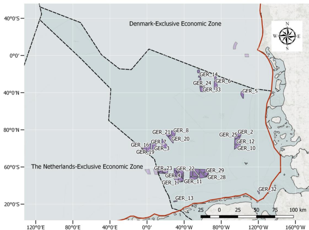
Fig. F2. OWF database – German EEZ
