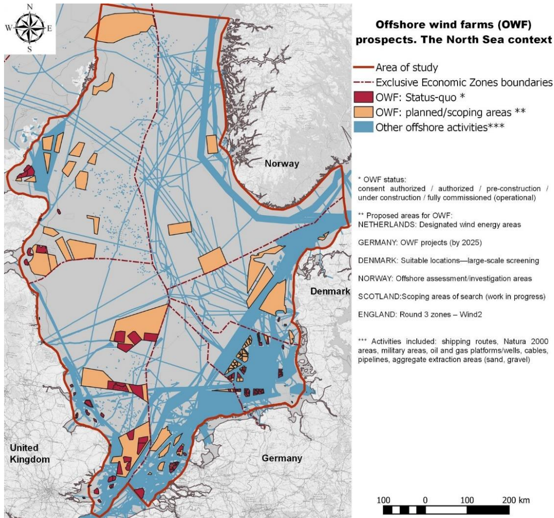
Figure 6. Offshore wind farm prospects (existing / authorised/planned) in the North Sea basin
