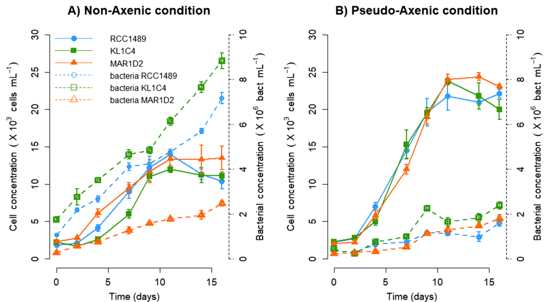
Figure 1. Lepidodinium chlorophorum concentrations (cell \text{mL}^{-1} ; solid lines) and bacterial concentrations (bacterial cell \text{mL}^{-1} ; dashed lines) for the three L. chlorophorum strains analysed under (A) non-axenic (NA) and (B) pseudo-axenic (PA) culture conditions. Symbols represent means and error bars represent the standard deviations from triplicate cultures.
