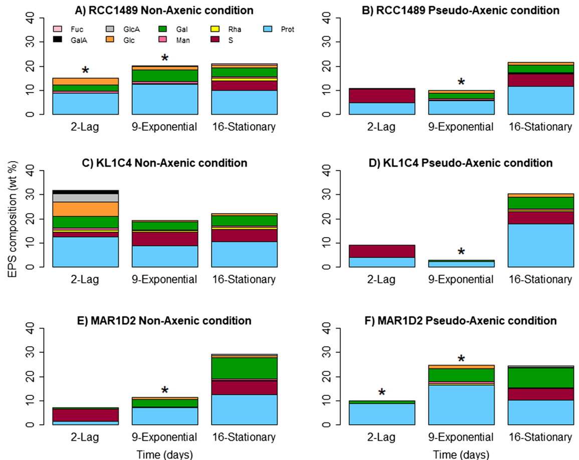
Figure 3. Monosaccharide composition, proteins and sulphate (wt %) of SEP from supernatants, at three growth times, for all three L. chlorophorum strains under non-axenic (NA) conditions: (A) RCC1489, (C) KL1C4, (E) MAR1D2 and pseudo-axenic (PA) conditions: (B) RCC1489, (D) KL1C4, (F) MAR1D2 (n = 1). Prot proteins, S sulphur, Rha rhamnose, Man mannose, Gal galactose, Glc glucose, GlcA glucuronic acid, GalA galacturonic acid, Fuc fucose. *Samples were not analysed for their sulphur content due to insufficient sample amount for elementary analysis.
