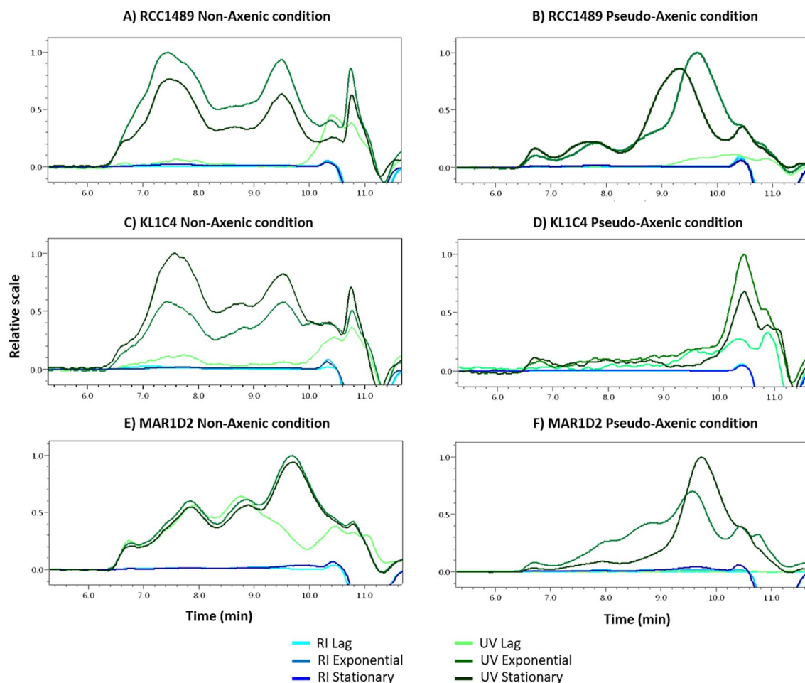
Figure 4. HPLC profiles (with UV and RI detectors) of culture supernatants obtained for three L. chlorophorum strains, at three growth times, under non-axenic (NA) conditions: (A) RCC1489, (C) KL1C4, (E) MAR1D2 and pseudo-axenic (PA) conditions: (B) RCC1489, (D) KL1C4, (F) MAR1D2 [Astra 6.1 Software (WYATT TECHNOLOGY)].
