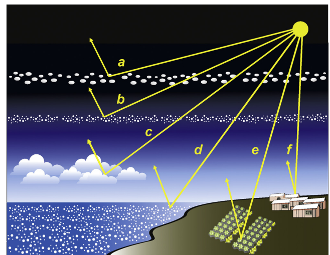
Fig. 1. Schematic diagram illustrating solar geoengineering approaches, a—using space mirrors, b—injecting aerosols into the stratosphere, c—brightening marine clouds, d—making the ocean surface more reflective, e—growing more reflective plants, and f—whitening roofs and other built structures (Caldeira et al., 2013).
