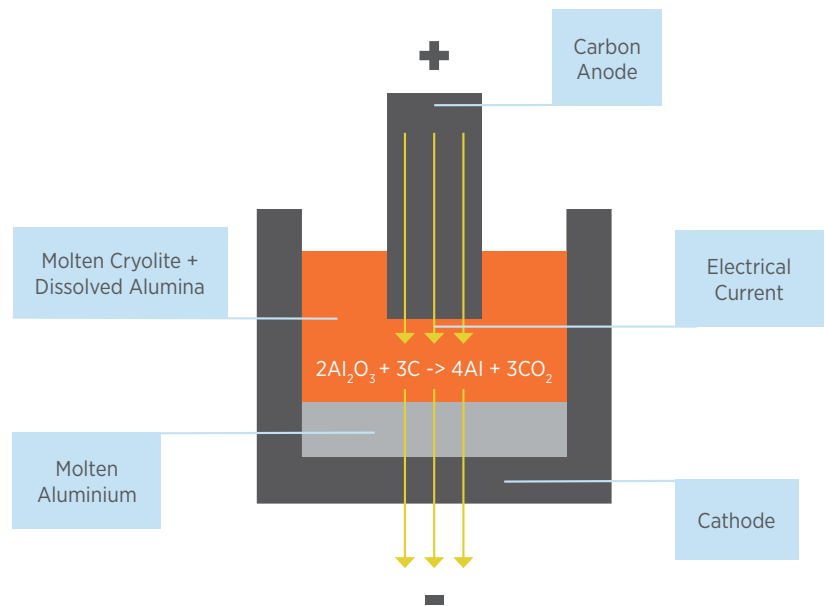
FIGURE 30: Schematic representation of the Hall-Hérout process
