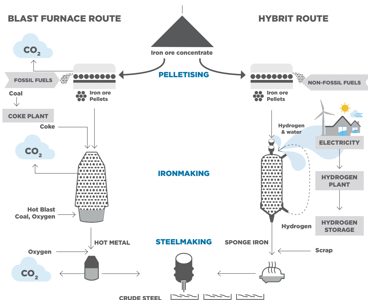
FIGURE 11: Renewable hydrogen-based DRI-EAF route piloted in Sweden compared to the conventional BF-BOF route
