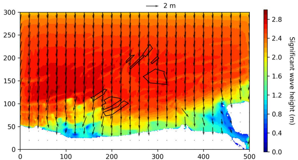
Figure 14: Significant wave height with boundaries at N, E and W. Waves at boundaries: H_s=2.0 m, T_p=7 s, Dir=NNW ; wind speed W_s=14 m/s.
