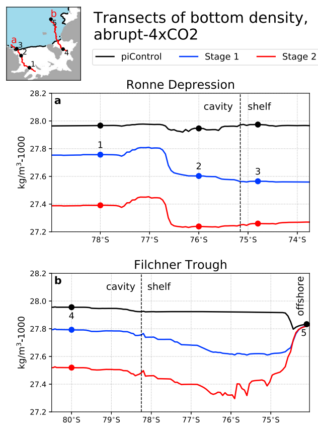
Fig. 4 Transects of potential density at the bottom of the water column in the FRIS cavity and surrounding continental shelf. a Ronne Depression; b Filchner Trough. The transects are shown in the inset map and consist of the points with the deepest bathymetry at each model latitude, within the given regions. The transects are shown averaged over three time periods: the entire piControl simulation (black), Stage 1 of the abrupt-4xCO 2 simulation (years 0–78; blue), and Stage 2 of the abrupt-4xCO 2 simulation (years 79–149; red). The points 1–5, as referenced in the text, are marked on both the density plots and the map. The dashed vertical line in each panel shows the location of the ice front. South of this line is the ice shelf cavity, and north of this line is the continental shelf. A small amount of the continental slope and offshore region is shown in the northernmost extent of (b).
