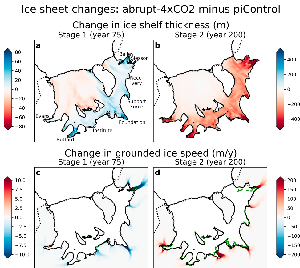
Fig. 7 Changes in ice sheet properties during the abrupt-4xCO 2 simulation and 50-year extension. a Ice shelf thickness anomaly (m) after 75 years; b after 200 years. c Grounded ice speed anomaly (m/y) after 75 years; d after 200 years. Note the differing colour scales for the two time periods. Model drift is removed by subtracting the piControl simulation at the same point in time. Black grounding lines are from the abrupt-4xCO 2 simulation, while the green contours in (c) and (d) show the piControl grounding lines for comparison. Pinning points in the Filchner Ice Shelf appear as isolated green points. Black labels in (a) denote geographical features: the Bailey, Foundation, Institute, Rutford, and Evans Ice Streams; and Slessor, Recovery, and Support Force Glaciers.
