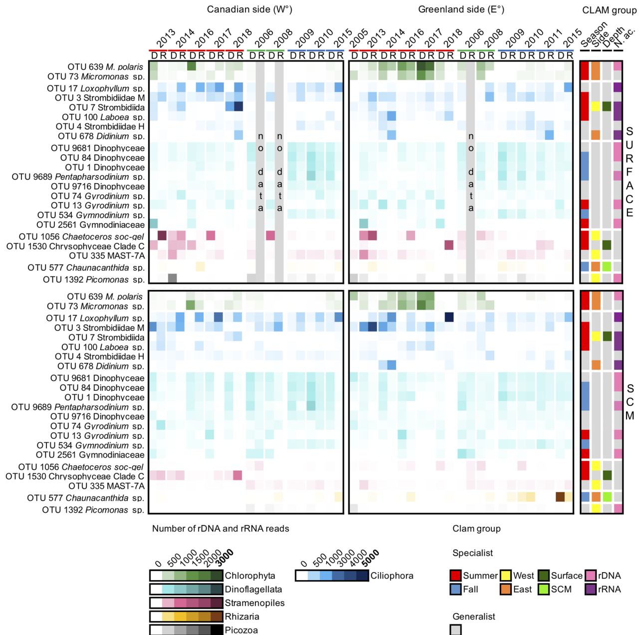
Figure 6. Proportion of reads from the 22 "top" OTUs defined as having reads accounting for >0.5% of the entire community. Samples are ordered chronologically for each season (July–August: 2005, 2013–2014, 2016–2018; September: 2006 and 2008; October: 2009–2011 and 2015). The heatmap shows the rRNA (R) and rDNA (D) library results (upper axis). Taxa are ordered and color coded by major high-level classification (approximately equivalent to phyla in botanical nomenclature): from most to least abundant in terms of reads within the phyla (see Fig. 7 for identification of the OTUs). The color intensity in the heatmap reflects the number of reads of each taxon with darker intensities indicating higher read counts, note the different scale for Ciliophora. Based on the results of CLAM test (Fig. 5; Supplementary Figs. S5, S6 and S7), the corner right bars indicate specialist taxa. Color coded for specificity to a season, a region, a depth or to nucleic acid source. Grey in all bars indicate non-specialist taxa for the category.
