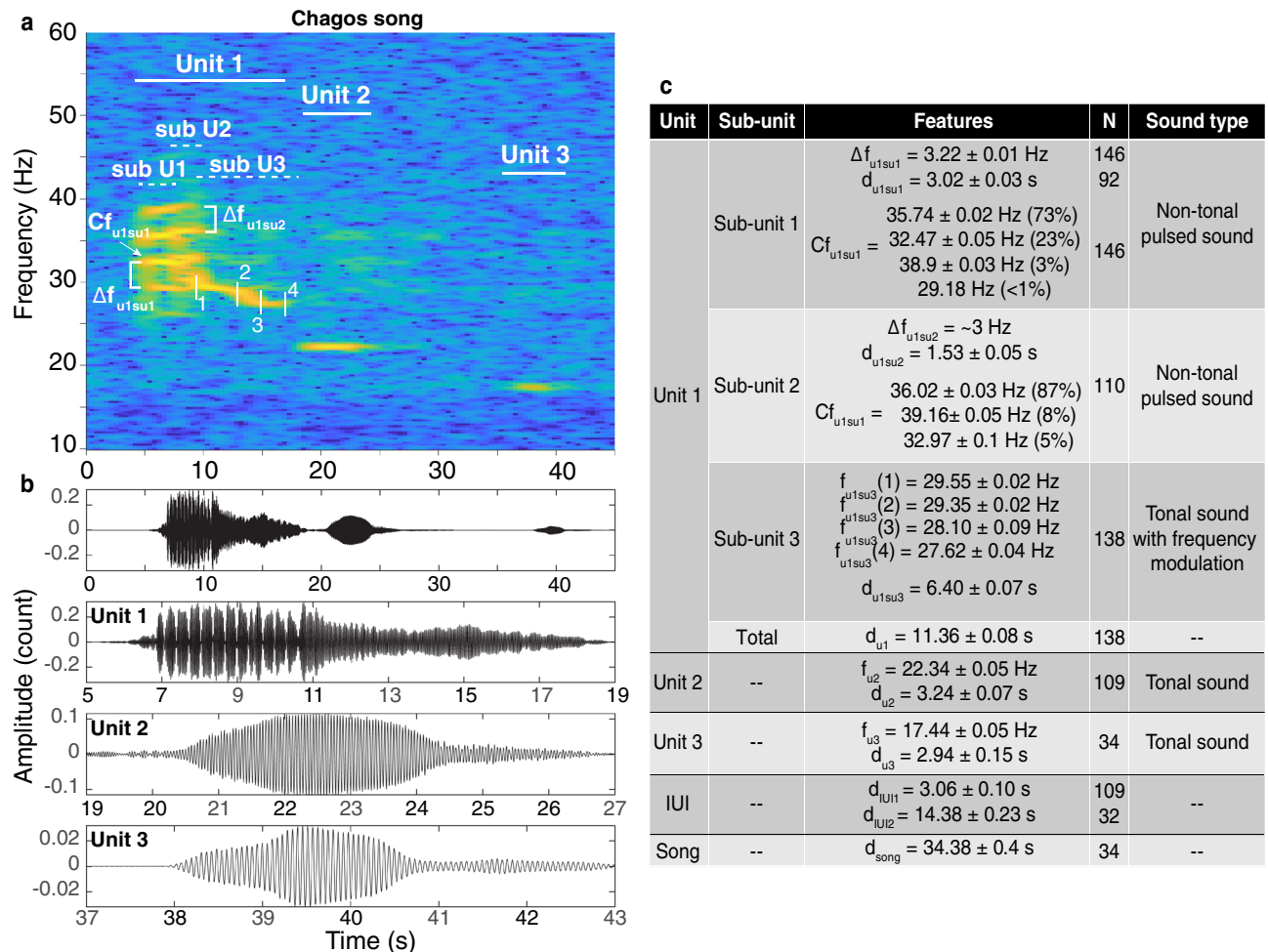
Figure 3. Spectrogram (a) and waveforms (b) of a Chagos song recorded on the eastern side of the Chagos Archipelago (DGS) in August 2017. Detailed waveforms show the signal structure of the units within the song. Spectrogram parameters: Hamming window, 1024-point FFT length, 90% overlap. Note that the axes differ among plots. (c) Measurements (mean \pm standard error (s.e.)) of the acoustic features. N is the number of measurements, u_i su_j stands for unit_i subunit_j where i and j are the unit and subunit numbers, \Delta f designates the frequency difference between the sidebands, f and d are the frequency and duration of the feature indicated in subscript, and when present, the number in brackets refers to the point measured as indicated on the spectrogram. F_x or G_x designate the x th harmonic of a sound, and Cf designates the carrier frequency of a sound.
