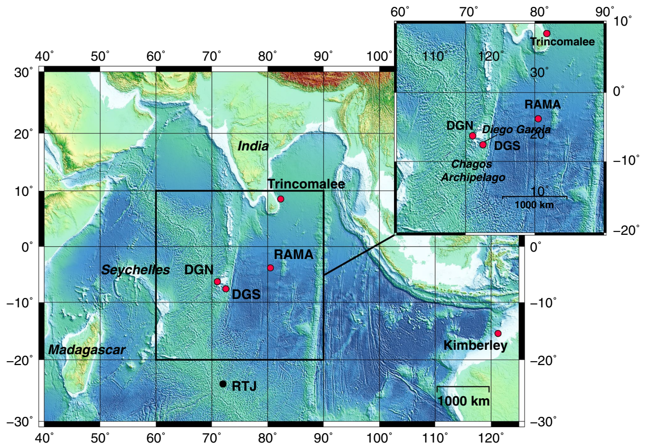
Figure 2. Study area and locations of the hydroacoustic stations (circles) used in this study to explore the presence of Chagos songs: in the equatorial waters, off Trincomalee, Sri Lanka; in the tropical waters: RAMA and the western (DGN) and eastern (DGS) sides of Chagos Archipelago; Kimberley, at the north of Western Australia, at the limit between the tropical and subtropical waters; and RTJ in the subtropical waters of the central Indian Ocean. Red circles indicate the sites where Chagos songs have been recorded.
