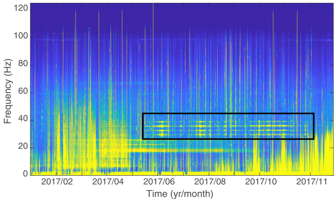
Figure 1. Long-term spectrogram of data recorded on the eastern side of the Chagos Archipelago (DGS site) in 2017: Chagos songs are a major component of the central Indian Ocean underwater soundscape and have been so for nearly two decades. The acoustic energy in the parallel horizontal frequency bands outlined in the black box are Chagos songs. Spectrogram parameters: 6 h averaging window, 50% overlap, FFT window of 120 s.
