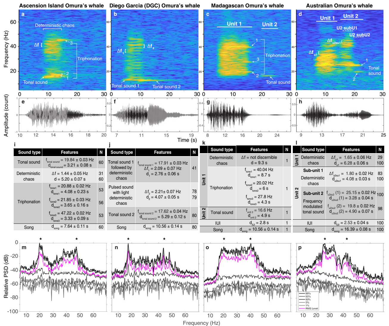
Figure 6. Spectrograms (a–d), waveforms (e–h), acoustic measurements (mean ± s.e.)—(i–l), and Power Spectral Density (PSD—m–p) of the songs of the Omura's whales from Ascension Island, Madagascar, Diego Garcia and Australia. The stars on the PSD (m–p) outline the peaks of energy. The Ascension Island song was recorded off Ascension Island (CTBTO records, site H10N1) in November 2005, the Madagascar song was recorded off Madagascar in December 2015 and provided by S. Cerchio, the Diego Garcia DGC song was recorded at DGN (CTBTO records, site H08N1) in October 2003 and the Australian song was recorded at Kimberley site in March 2013 (IMOS records). For the panels (a–d) and (i–j): N is the number of measurements, u_i stands for unit/subunit; where i and j are the unit and subunit measurements, \Delta f designates the frequency difference between the sidebands, f and d are the frequency and duration of the feature indicated in subscript, and when present, the number in brackets refers to the point measured as indicated on the corresponding spectrogram. (Spectrogram parameters: Hamming window, 1024-point FFT length, 90% overlap. Note that the axes differ among plots).
