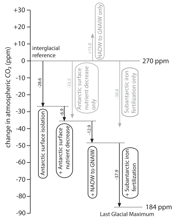
Fig. 2. Simulated changes in the concentration of atmospheric CO 2 (in parts per million by volume, ppm) due to proposed ice age changes in the Southern Ocean as well as in the character of North Atlantic-formed deep water (from Hain et al., 2010). NADW and GNAIW refer to North Atlantic Deep Water and Glacial North Atlantic Intermediate Water. The interglacial reference case of the model has an atmospheric CO 2 concentration of 270 ppm. The gray arrows indicate the CO 2 change caused by a given forcing if active by itself, whereas the black arrows indicate successive addition of forcings from left to right. First, AZ surface isolation, removing essentially all deep ventilation from the AZ surface, causes a CO 2 decline of 29 ppm. In these experiments, the only water exchanges that are reduced are those related to ventilation of the "lower cell" of Southern Ocean overturning (i.e., AZ-formed deep water); this strategy was taken to distinguish the CO 2 effect of AZ surface isolation from that of reducing the nutrient supply to SAZ surface waters. Second, AZ surface nutrient concentration is lowered to ~50% of its interglacial value. If conducted alone, without AZ surface isolation, the nutrient drawdown causes a 33 ppm decline; however, without a circulation change, a nutrient drawdown would require an increase in export production, counter to ice age observations (e.g., Jaccard et al., 2013). In contrast to its effect when applied alone, when nutrient drawdown is applied in concert with AZ surface isolation, it only contributes an additional 7 ppm decline beyond the 29 ppm from AZ surface isolation. Again, in these experiments, this is implemented in a way that SAZ surface nutrients are not affected. Third, a shift from the formation of NADW to GNAIW, when conducted in the context of the first two changes, contributes an additional 13 ppm decline. In contrast, when the change to GNAIW is conducted alone, without the Southern Ocean changes, it raises atmospheric CO 2 by 16 ppm because it gives over more of the ocean interior to ventilation by the high-nutrient AZ. SAZ iron fertilization (implemented as an export production increase that causes a ~43% decline in SAZ surface nutrient concentration) lowers atmospheric CO 2 by 38 ppm, whether it is conducted alone or in combination with any of the other changes. The AZ surface is an important source of nutrients to the SAZ. If, in the model, AZ nutrient drawdown is allowed to cause nutrient decline in the SAZ as well, then the AZ changes lower CO 2 more than indicated here, while the SAZ iron fertilization lowers CO 2 correspondingly less, resulting in no change in the net CO 2 decline from the combined forcings. A CO 2 decline of 86 ppm occurs from simultaneous implementation of all four changes, producing an atmospheric CO 2 concentration of 184 ppm, which is similar to observations for the LGM. LGM conditions for the temperature, salinity, and volume of the ocean are not implemented here and in combination may have reduced ice age CO 2 by an additional ~30 ppm (Kohfeld and Ridgwell, 2009); the simulations described here were for an isothermal ocean, such that imposed circulation changes did not alter the average ocean temperature. There is also no implementation of an ice age decline in the terrestrial biosphere and soil carbon inventories, which may have raised atmospheric CO 2 by ~15 ppm (Sigman and Boyle, 2000).
