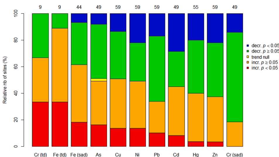
Fig. 3. Relative proportions of sites monitored for each TE over a minimum of six years, which show a net increase (incr. p < 0.05 , red) or decrease (decr. p < 0.05 , blue), an increase (incr. p \geq 0.05 , orange) or decrease (decr. p \geq 0.05 , green) or no evolution (trend null, yellow) of their sediment TE concentrations. Numbers above bars are number of sites included in the median regression analysis. Digestion techniques: strong acid digestion (sad) or total digestion (td) are specified and considered separately for Cr and Fe. (For interpretation of the references to colour in this figure legend, the reader is referred to the web version of this article.)
