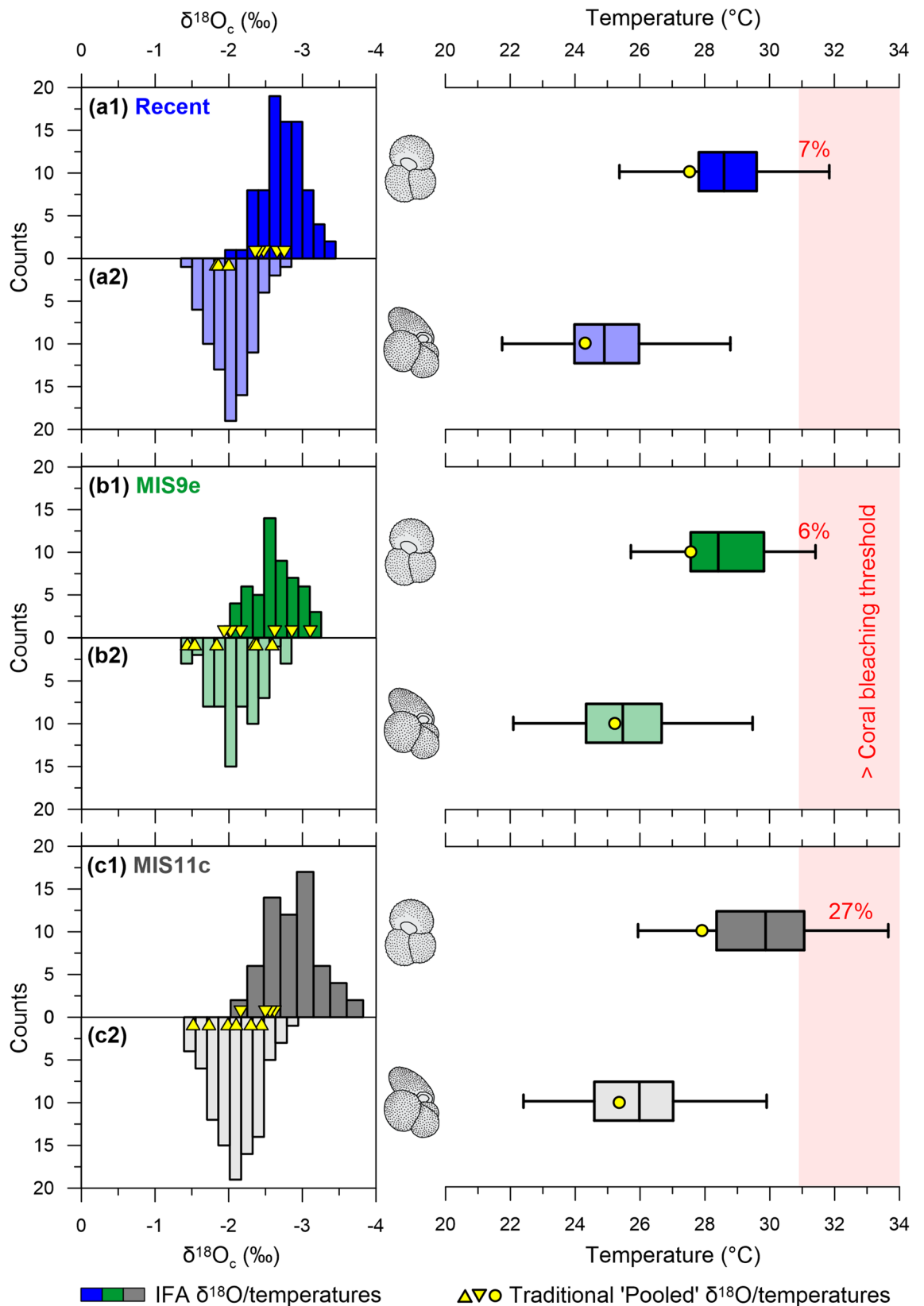
Figure 4. Spread in \delta^{18}\text{O}_c individual foraminiferal analysis (IFA) data and seawater temperature estimates. Histograms of the \delta^{18}\text{O}_c IFA data spread (counts = number of measurements) and the corresponding temperatures (box and whisker plots) for (a) the Recent (blue), (b) MIS9e (green) and (c) MIS11c (grey) for both (1) G. ruber (w) and (2) T. sacculifer (w/s). Traditional \delta^{18}\text{O}_c values (based on pooled specimens) (yellow triangles) are shown for each sample together with the mean \delta^{18}\text{O} derived temperature (based on pooled specimens) (yellow circles). Temperatures > the Maldives coral bleaching threshold (~30.9 °C 10 ) are shown in red shading. Numbers indicate the percentage of the IFA temperature estimates, from each dataset, > this bleaching threshold. Note: MIS9e and MIS11c represent the pooled data from three samples.
