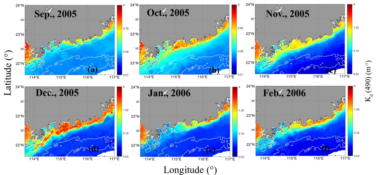
Figure 10. The monthly mean K_d(490) values ( \text{m}^{-1} ) from September 2005 to February 2006. The program R (version 3.6.3, available at https://www.r-project.org ) was applied for the map.
