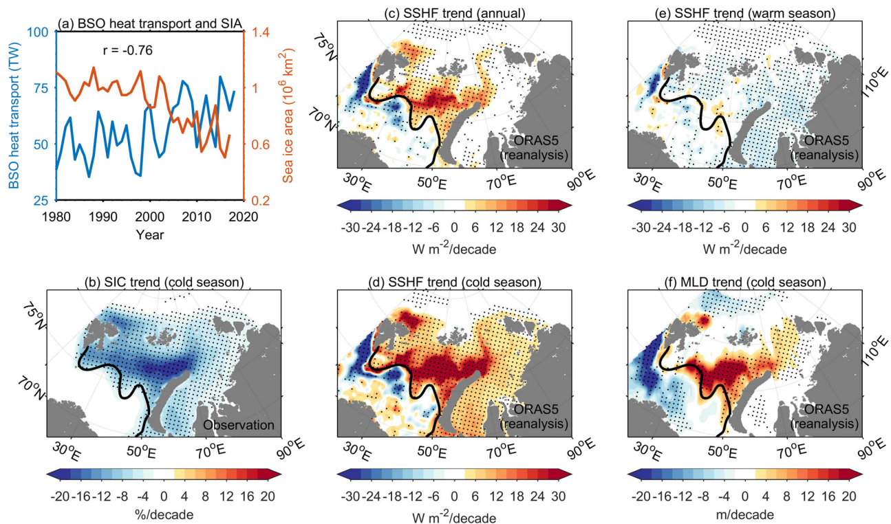
Fig. 1 Climate change in the Barents and Kara Seas in the past. a The time series of ocean heat transport through the Barents Sea Opening (BSO) and the cold season (October–March) sea ice area (SIA) in the Barents and Kara Seas. The linear trends of b cold season sea ice concentration (SIC), c annual mean sea surface heat flux (SSHF), d cold season sea surface heat flux, e warm season (April–September) sea surface heat flux, and f cold season mixed layer depth (MLD) of 1979/80–2017/18. Dots indicate that linear trends exceeded the 95% confidence level. The black lines in b–f are the 0 °C surface isotherm based on climatology from WOA13, which can represent the boundary between the southwestern and northern Barents Sea 14 . Upward sea surface heat flux is positive. Ocean heat transport ( a ), SSHF ( c , e , d ), and MLD ( f ) are from the Ocean ReAnalysis System 5 (ORAS5). Satellite observed SIA ( a ) and SIC ( b ) are from the National Snow and Ice Data Center.
