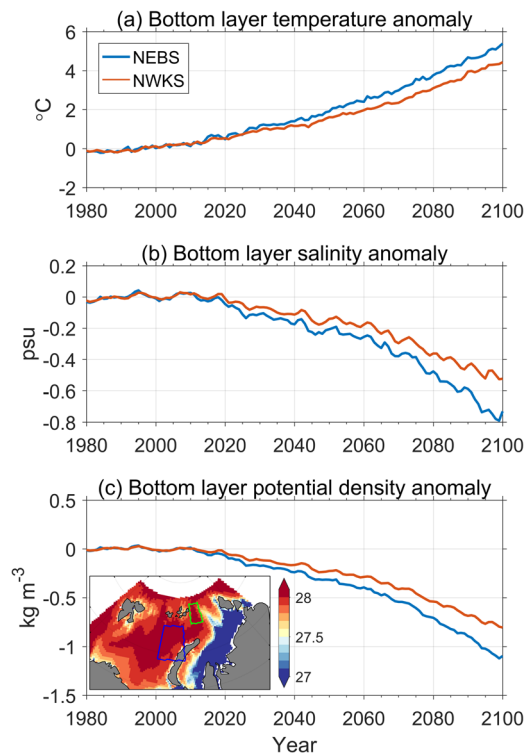
Fig. 5 Climate change of Barents Sea Water. Anomalies of CMIP6 MMM bottom layer temperature (a), salinity (b), and potential density referenced to surface (c) in the northeastern Barents Sea (NEBS) and northwestern Kara Sea (NWKS). Anomalies are referenced to the mean over the period 1979–2008. The insert panel in c depicts CMIP6 MMM climatology of bottom layer potential density averaged over the period of 1979–2018. The blue and green boxes in the insert panel in c represent the NEBS and NWKS, respectively.
