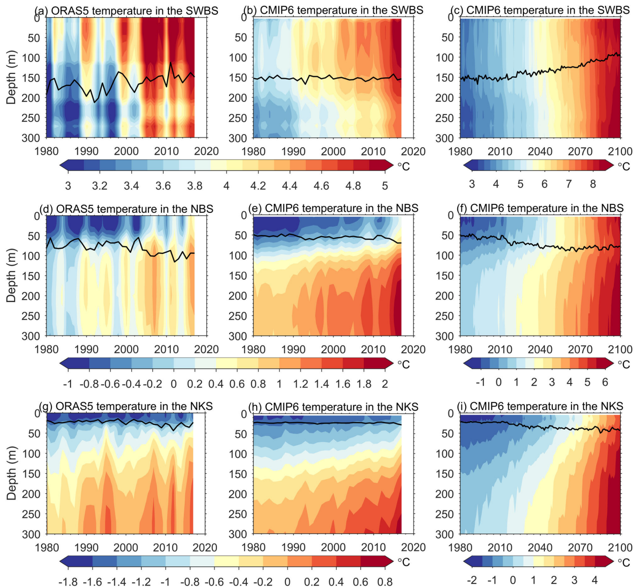
Fig. 3 Temperature changes in the southwestern Barents Sea, northern Barents Sea, and northern Kara Sea. a–c Depth-time plots of cold season temperature averaged in the southwestern Barents Sea (SWBS, the red box shown in Fig. 2a) in the reanalysis (ORAS5) and CMIP6 MMM. d–f The same as a–c , but for the northern Barents Sea (NBS, the black box shown in Fig. 2a). g–i The same as a–c , but for the northern Kara Sea (NKS, the magenta box shown in Fig. 2a). The black lines show the mixed layer depth (MLD) averaged in the respective boxes.
