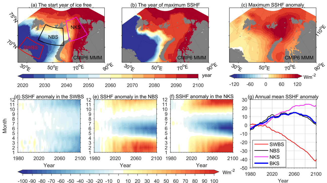
Fig. 4 The temporal and spatial evolution of the Arctic Ocean cooling machine. a The start year of being ice-free in the cold season during 2018/19–2099/2100. b The year of maximum cold-season sea surface heat flux (SSHf) anomalies during 2018/19–2099/2100. c The maximum of cold-season sea surface heat flux anomalies during 2018/19–2099/2100 referenced to the climatology. d–f Thirteen-year smoothed monthly sea surface heat flux anomalies averaged in the southwestern Barents Sea (SWBS), northern Barents and Kara Seas (NBS and NKS). g Thirteen-year smoothed annual mean sea surface heat flux anomalies averaged in the SWBS, NBS, NKS, and the entire Barents and Kara Seas (BKS). Anomalies are referenced to the mean over the period 1979–2008. The red, black, and magenta boxes in a indicate the areas used in d , e , and f , respectively.
