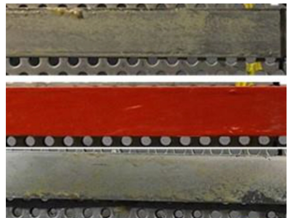
Fig. 9. Steel stripes after freshwater exposure of run 2, before water jet cleaning. From top: steel, FR2, SiPEG20i.
