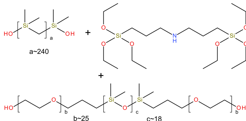
Fig. 2. Main components of the SiPEG coatings.
